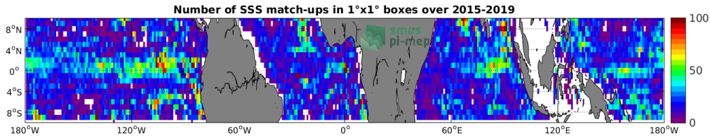
Figure 4: Number of SSS match-ups between Argo SSS and the SMAP-L3-RSS-V4-8DAY-RUNNING SSS product for the Equatorial Ocean 10N-10S Pi-MEP region over 1^\circ \times 1^\circ boxes and for the full satellite product period.
