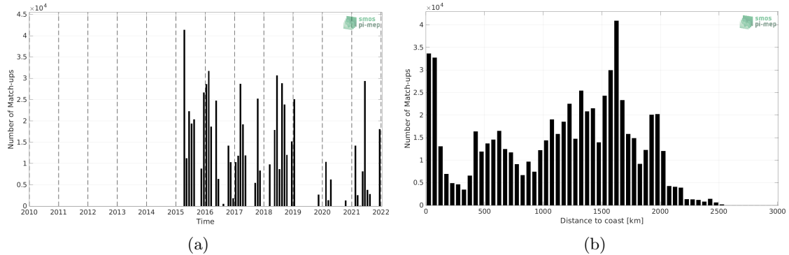
Figure 1: Number of match-ups between TSG (SAMOS) and SMAP SSS L3 v4 - Monthly (RSS) SSS as a function of time (a) and as function of the distance to coast (b) over the Equatorial Ocean 10N-10S Pi-MEP region and for the full satellite product period.
