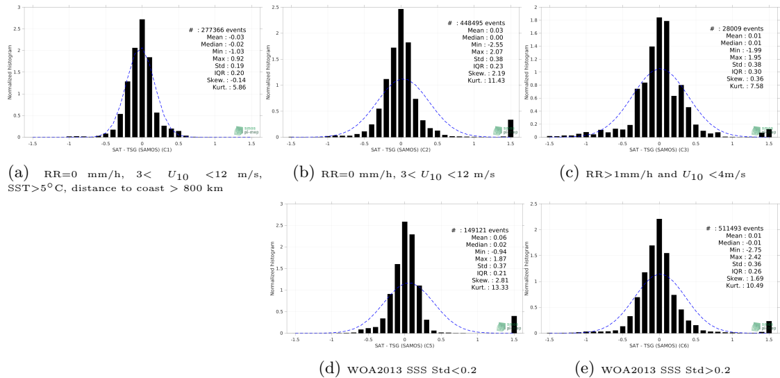
Figure 13: Normalized histogram of \Delta SSS (SMAP SSS L3 v4 - Monthly (RSS) - TSG (SAMOS)) for 5 different subdatasets corresponding to: RR=0 mm/h, 3 < U_{10} < 12 m/s, SST > 5^\circ C , distance to coast > 800 km (a), RR=0 mm/h, 3 < U_{10} < 12 m/s (b), RR>1mm/h and U_{10} < 4 m/s (c), WOA2013 SSS Std<0.2 (d), WOA2013 SSS Std>0.2 (e).
