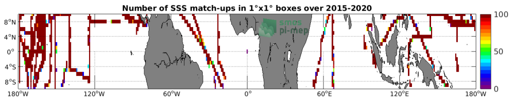
Figure 4: Number of SSS match-ups between TSG (SAMOS) SSS and the SMAP SSS L3 v4 - Monthly (RSS) SSS product for the Equatorial Ocean 10N-10S Pi-MEP region over 1°x1° boxes and for the full satellite product period.
