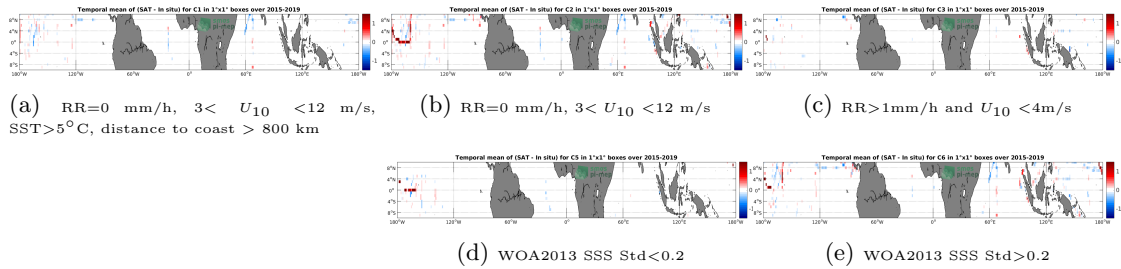
Figure 12: Temporal mean gridded over spatial boxes of size 1°x1° of ΔSSS (SMAP-L3-RSS-V4-MONTHLY - TSG-SAMOS) for 5 different subdatasets corresponding to:RR=0 mm/h, 3< U 10 <12 m/s, SST>5°C, distance to coast > 800 km (a), RR=0 mm/h, 3< U 10 <12 m/s (b), RR>1mm/h and U 10 <4m/s (c), WOA2013 SSS Std<0.2 (d), WOA2013 SSS Std>0.2 (e).
