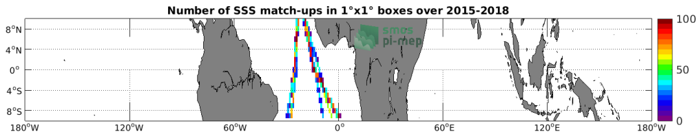
Figure 4: Number of SSS match-ups between TSG (Polarstern) SSS and the SMAP SSS L3 v4 - Monthly (RSS) SSS product for the Equatorial Ocean 10N-10S Pi-MEP region over 1°x1° boxes and for the full satellite product period.
