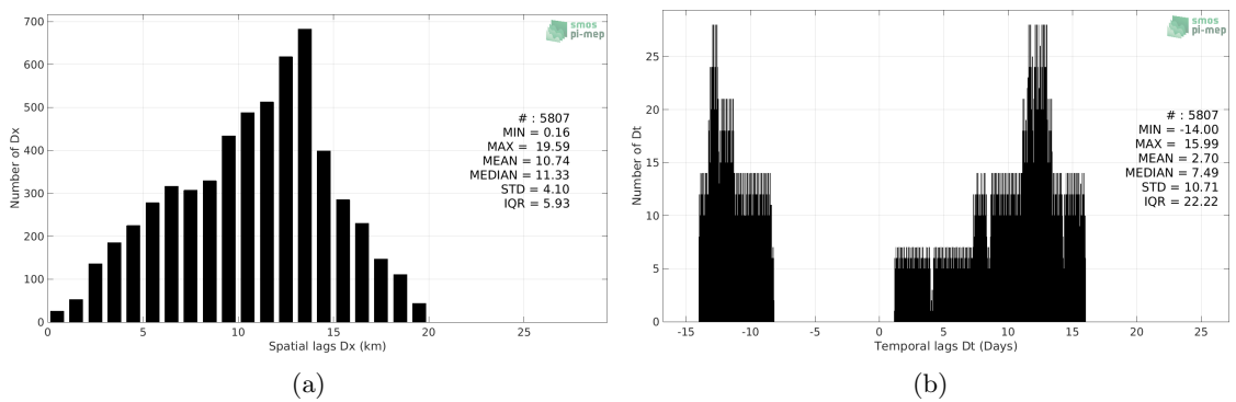
Figure 5: Histograms of the spatial (a) and temporal (b) lags between the time of the TSG (Polarstern) measurements and the date of the corresponding SMAP SSS L3 v4 - Monthly (RSS) SSS product.
