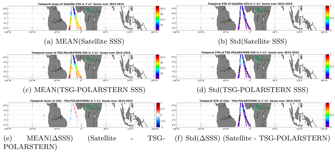
Figure 6: Temporal mean (left) and Std (right) of SSS from SMAP-L3-RSS-V4-MONTHLY (top), TSG-POLARSTERN (middle), and of \Delta SSS (Satellite - TSG-POLARSTERN). Only match-up pairs are used to generate these maps.
