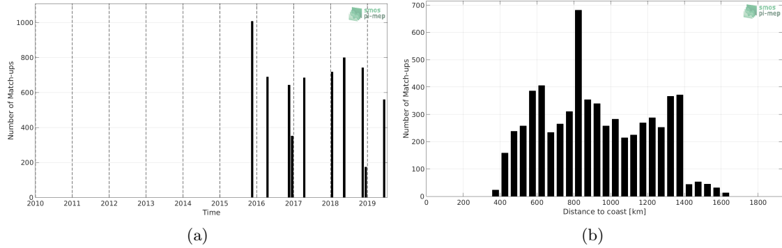
Figure 1: Number of match-ups between TSG-POLARSTERN and SMAP-L3-RSS-V4-MONTHLY SSS as a function of time (a) and as function of the distance to coast (b) over the Equatorial Ocean 10N-10S Pi-MEP region and for the full satellite product period.
