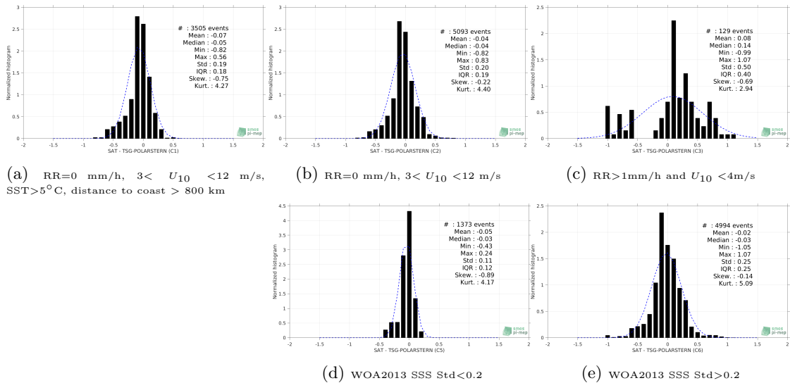
Figure 13: Normalized histogram of ΔSSS (SMAP-L3-RSS-V4-MONTHLY - TSG-POLARSTERN) for 5 different subdatasets corresponding to: RR=0 mm/h, 3 < U 10 < 12 m/s, SST > 5°C, distance to coast > 800 km (a), RR=0 mm/h, 3 < U 10 < 12 m/s (b), RR > 1mm/h and U 10 < 4m/s (c), WOA2013 SSS Std < 0.2 (d), WOA2013 SSS Std > 0.2 (e).
