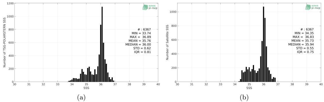
Figure 2: Histograms of SSS from TSG-POLARSTERN (a) and SMAP-L3-RSS-V4-MONTHLY (b) considering all match-up pairs per bins of 0.1 over the Equatorial Ocean 10N-10S Pi-MEP region and for the full satellite product period.
