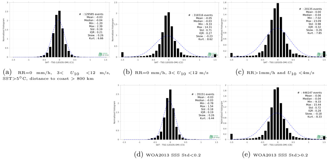
Figure 13: Normalized histogram of \Delta SSS (SMAP SSS L3 v4 - Monthly (RSS) - TSG (LEGOS-DM)) for 5 different subdatasets corresponding to: RR=0 mm/h, 3 < U_{10} < 12 m/s, SST >5^\circ C, distance to coast > 800 km (a), RR=0 mm/h, 3 < U_{10} < 12 m/s (b), RR >1 mm/h and U_{10} < 4 m/s (c), WOA2013 SSS Std <0.2 (d), WOA2013 SSS Std >0.2 (e).
