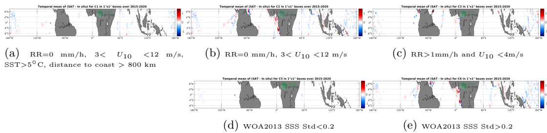
Figure 12: Temporal mean gridded over spatial boxes of size 1^\circ \times 1^\circ of \Delta SSS (SMAP SSS L3 v4 - Monthly (RSS) - TSG (LEGOS-DM)) for 5 different subdatasets corresponding to:RR=0 mm/h, 3 < U_{10} < 12 m/s, SST>5°C, distance to coast > 800 km (a), RR=0 mm/h, 3 < U_{10} < 12 m/s (b), RR>1mm/h and U_{10} < 4 m/s (c), WOA2013 SSS Std<0.2 (d), WOA2013 SSS Std>0.2 (e).
