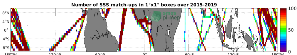
Figure 4: Number of SSS match-ups between TSG (LEGOS-DM) SSS and the SMAP SSS L3 v4 - Monthly (RSS) SSS product for the Equatorial Ocean 10N-10S Pi-MEP region over 1°x1° boxes and for the full satellite product period.
