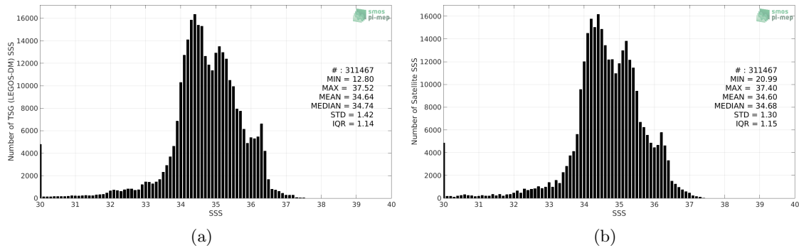
Figure 2: Histograms of SSS from TSG (LEGOS-DM) (a) and SMAP SSS L3 v4 - Monthly (RSS) (b) considering all match-up pairs per bins of 0.1 over the Equatorial Ocean 10N-10S Pi-MEP region and for the full satellite product period.
