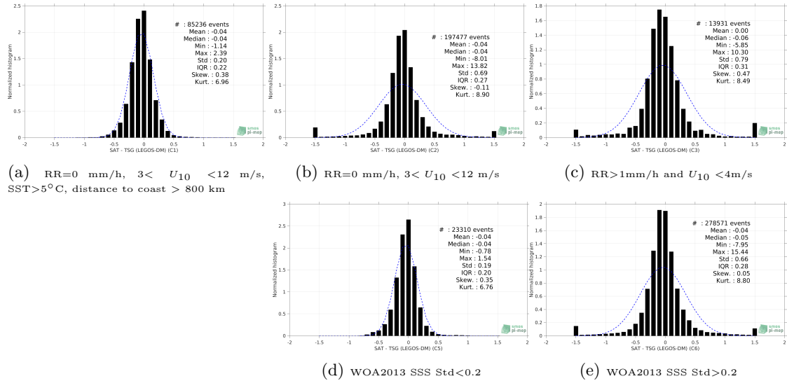
Figure 13: Normalized histogram of \Delta SSS (SMAP SSS L3 v4 - Monthly (RSS) - TSG (LEGOS-DM)) for 5 different subdatasets corresponding to: RR=0 mm/h, 3 < U_{10} < 12 m/s, SST > 5^\circ C , distance to coast > 800 km (a), RR=0 mm/h, 3 < U_{10} < 12 m/s (b), RR>1mm/h and U_{10} < 4 m/s (c), WOA2013 SSS Std<0.2 (d), WOA2013 SSS Std>0.2 (e).
