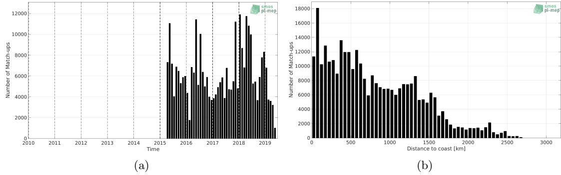
Figure 1: Number of match-ups between TSG (LEGOS-DM) and SMAP SSS L3 v4 - Monthly (RSS) SSS as a function of time (a) and as function of the distance to coast (b) over the Equatorial Ocean 10N-10S Pi-MEP region and for the full satellite product period.
