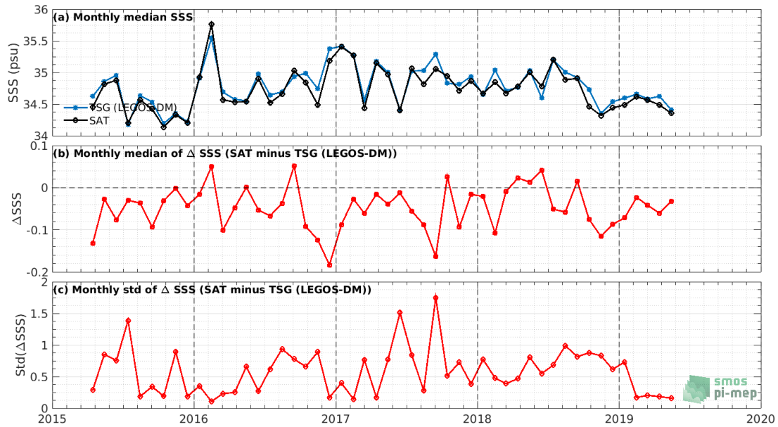
Figure 7: Time series of the monthly median SSS (top), median of \Delta SSS (Satellite - TSG (LEGOS-DM)) and Std(\Delta SSS) (Satellite - TSG (LEGOS-DM)) over the Equatorial Ocean 10N-10S Pi-MEP region considering all match-ups collected by the Pi-MEP.
