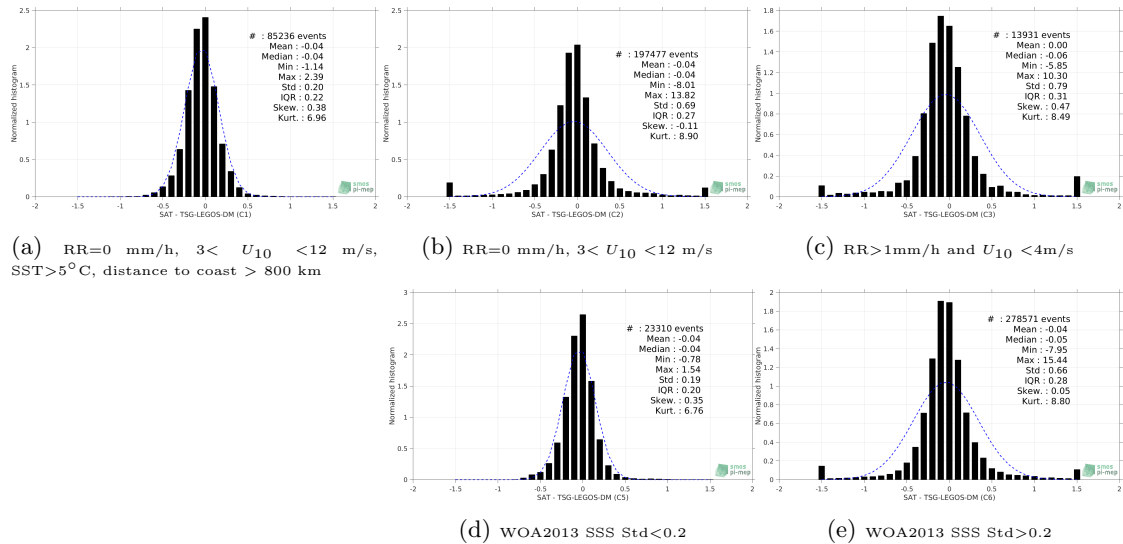
Figure 13: Normalized histogram of \Delta SSS (SMAP-L3-RSS-V4-MONTHLY - TSG-LEGOS-DM) for 5 different subdatasets corresponding to: RR=0 mm/h, 3 < U_{10} < 12 m/s, SST >5^\circ\text{C} , distance to coast > 800 km (a), RR=0 mm/h, 3 < U_{10} < 12 m/s (b), RR >1 mm/h and U_{10} < 4 m/s (c), WOA2013 SSS Std <0.2 (d), WOA2013 SSS Std >0.2 (e).
