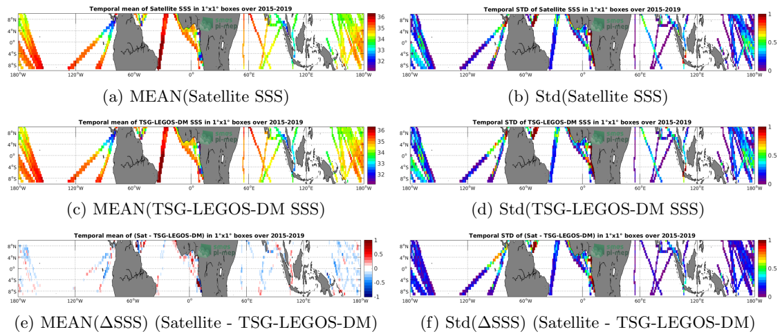
Figure 6: Temporal mean (left) and Std (right) of SSS from SMAP-L3-RSS-V4-MONTHLY (top), TSG-LEGOS-DM (middle), and of \Delta SSS (Satellite - TSG-LEGOS-DM). Only match-up pairs are used to generate these maps.
