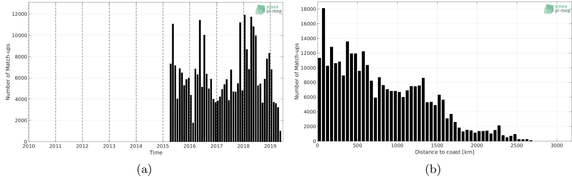
Figure 1: Number of match-ups between TSG-LEGOS-DM and SMAP-L3-RSS-V4-MONTHLY SSS as a function of time (a) and as function of the distance to coast (b) over the Equatorial Ocean 10N-10S Pi-MEP region and for the full satellite product period.
