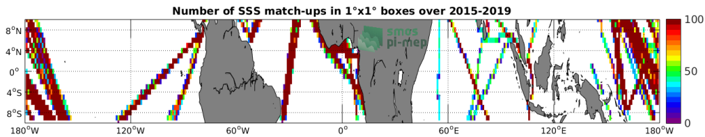
Figure 4: Number of SSS match-ups between TSG-LEGOS-DM SSS and the SMAP-L3-RSS-V4-MONTHLY SSS product for the Equatorial Ocean 10N-10S Pi-MEP region over 1°x1° boxes and for the full satellite product period.
