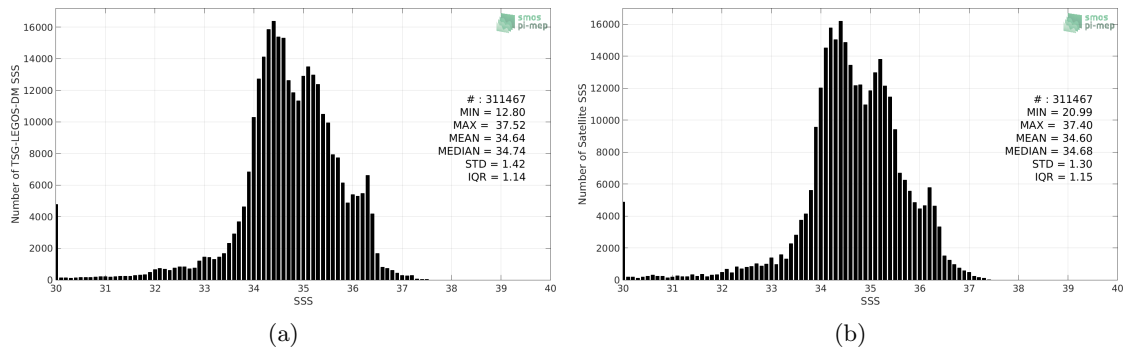
Figure 2: Histograms of SSS from TSG-LEGOS-DM (a) and SMAP-L3-RSS-V4-MONTHLY (b) considering all match-up pairs per bins of 0.1 over the Equatorial Ocean 10N-10S Pi-MEP region and for the full satellite product period.
