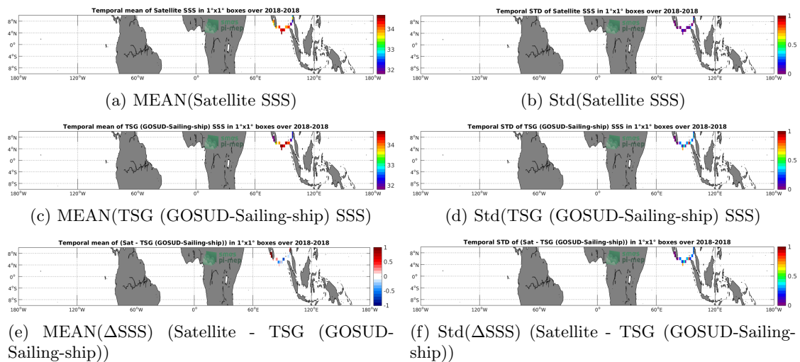
Figure 6: Temporal mean (left) and Std (right) of SSS from SMAP SSS L3 v4 - Monthly (RSS) (top), TSG (GOSUD-Sailing-ship) (middle), and of \Delta SSS (Satellite - TSG (GOSUD-Sailing-ship)). Only match-up pairs are used to generate these maps.
