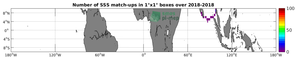
Figure 4: Number of SSS match-ups between TSG (GOSUD-Sailing-ship) SSS and the SMAP SSS L3 v4 - Monthly (RSS) SSS product for the Equatorial Ocean 10N-10S Pi-MEP region over 1^\circ \times 1^\circ boxes and for the full satellite product period.
