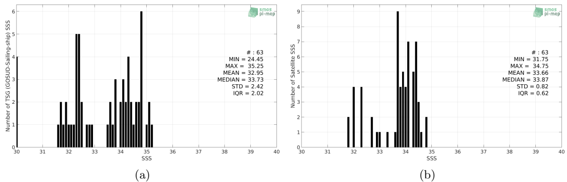
Figure 2: Histograms of SSS from TSG (GOSUD-Sailing-ship) (a) and SMAP SSS L3 v4 - Monthly (RSS) (b) considering all match-up pairs per bins of 0.1 over the Equatorial Ocean 10N-10S Pi-MEP region and for the full satellite product period.
