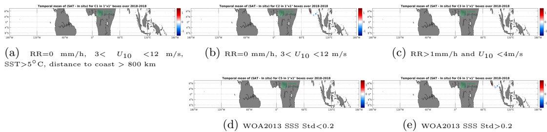
Figure 12: Temporal mean gridded over spatial boxes of size 1°x1° of \Delta SSS (SMAP SSS L3 v4 - Monthly (RSS) - TSG (GOSUD-Sailing-ship)) for 5 different subdatasets corresponding to: RR=0 mm/h, 3 < U_{10} < 12 m/s, SST>5°C, distance to coast > 800 km (a), RR=0 mm/h, 3 < U_{10} < 12 m/s (b), RR>1mm/h and U_{10} < 4 m/s (c), WOA2013 SSS Std<0.2 (d), WOA2013 SSS Std>0.2 (e).
