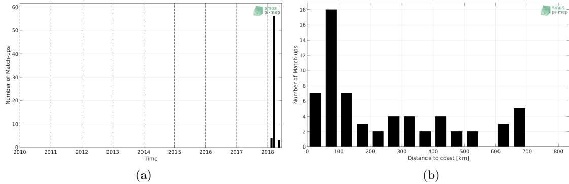
Figure 1: Number of match-ups between TSG (GOSUD-Sailing-ship) and SMAP SSS L3 v4 - Monthly (RSS) SSS as a function of time (a) and as function of the distance to coast (b) over the Equatorial Ocean 10N-10S Pi-MEP region and for the full satellite product period.
