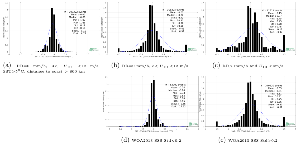
Figure 13: Normalized histogram of \Delta\text{SSS} (SMAP SSS L3 v4 - Monthly (RSS) - TSG (GOSUD-Research-vessel)) for 5 different subdatasets corresponding to: RR=0 mm/h, 3 < U_{10} < 12 m/s, SST>5°C, distance to coast > 800 km (a), RR=0 mm/h, 3 < U_{10} < 12 m/s (b), RR>1mm/h and U_{10} < 4 m/s (c), WOA2013 SSS Std<0.2 (d), WOA2013 SSS Std>0.2 (e).
