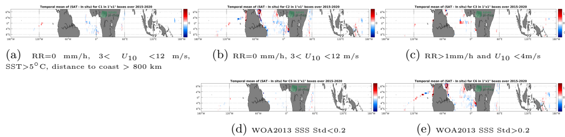
Figure 12: Temporal mean gridded over spatial boxes of size 1^\circ \times 1^\circ of \Delta\text{SSS} (SMAP SSS L3 v4 - Monthly (RSS) - TSG (GOSUD-Research-vessel)) for 5 different subdatasets corresponding to: RR=0 mm/h, 3 < U_{10} < 12 m/s, SST>5°C, distance to coast > 800 km (a), RR=0 mm/h, 3 < U_{10} < 12 m/s (b), RR>1mm/h and U_{10} < 4 m/s (c), WOA2013 SSS Std<0.2 (d), WOA2013 SSS Std>0.2 (e).
