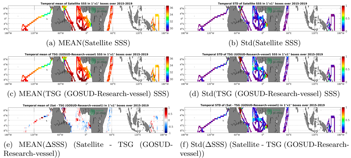
Figure 6: Temporal mean (left) and Std (right) of SSS from SMAP SSS L3 v4 - Monthly (RSS) (top), TSG (GOSUD-Research-vessel) (middle), and of \Delta SSS (Satellite - TSG (GOSUD-Research-vessel)). Only match-up pairs are used to generate these maps.
