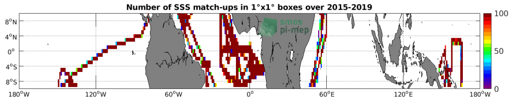
Figure 4: Number of SSS match-ups between TSG (GOSUD-Research-vessel) SSS and the SMAP SSS L3 v4 - Monthly (RSS) SSS product for the Equatorial Ocean 10N-10S Pi-MEP region over 1^\circ \times 1^\circ boxes and for the full satellite product period.
