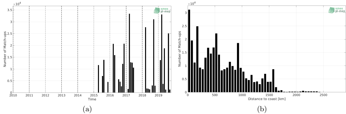
Figure 1: Number of match-ups between TSG (GOSUD-Research-vessel) and SMAP SSS L3 v4 - Monthly (RSS) SSS as a function of time (a) and as function of the distance to coast (b) over the Equatorial Ocean 10N-10S Pi-MEP region and for the full satellite product period.
