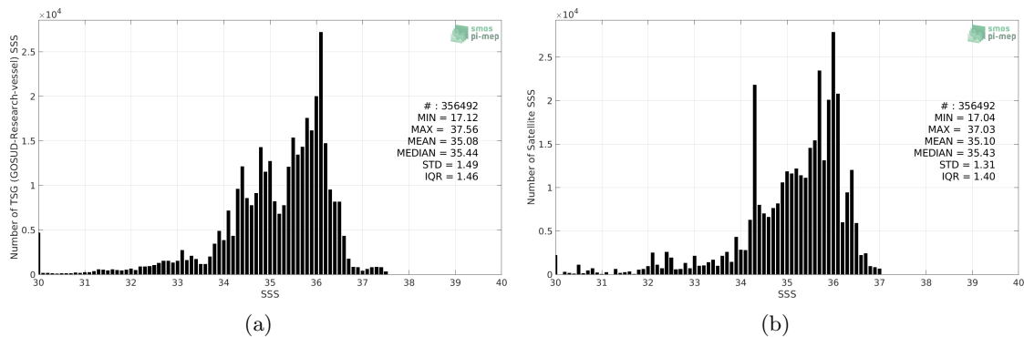
Figure 2: Histograms of SSS from TSG (GOSUD-Research-vessel) (a) and SMAP SSS L3 v4 - Monthly (RSS) (b) considering all match-up pairs per bins of 0.1 over the Equatorial Ocean 10N-10S Pi-MEP region and for the full satellite product period.
