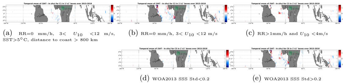
Figure 12: Temporal mean gridded over spatial boxes of size 1°x1° of ΔSSS (SMAP-L3-RSS-V4-MONTHLY - TSG-GOSUD-Research-vessel) for 5 different subdatasets corresponding to:RR=0 mm/h, 3 < U 10 < 12 m/s, SST>5°C, distance to coast > 800 km (a), RR=0 mm/h, 3 < U 10 < 12 m/s (b), RR>1mm/h and U 10 < 4m/s (c), WOA2013 SSS Std<0.2 (d), WOA2013 SSS Std>0.2 (e).
