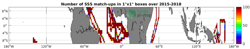
Figure 4: Number of SSS match-ups between TSG-GOSUD-Research-vessel SSS and the SMAP-L3-RSS-V4-MONTHLY SSS product for the Equatorial Ocean 10N-10S Pi-MEP region over 1^\circ \times 1^\circ boxes and for the full satellite product period.
