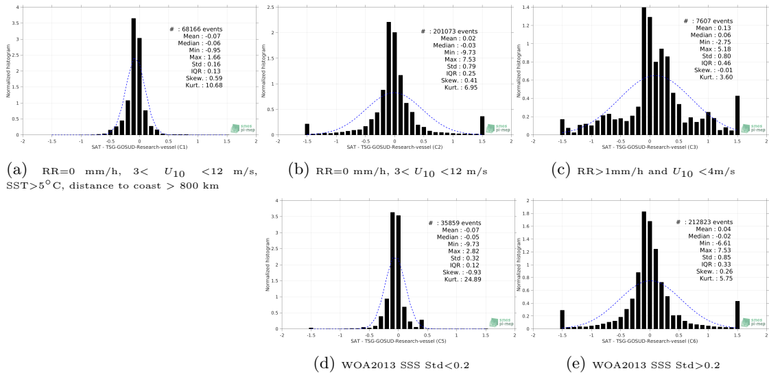
Figure 13: Normalized histogram of ΔSSS (SMAP-L3-RSS-V4-MONTHLY - TSG-GOSUD-Research-vessel) for 5 different subdatasets corresponding to: RR=0 mm/h, 3 < U 10 < 12 m/s, SST>5°C, distance to coast > 800 km (a), RR=0 mm/h, 3 < U 10 < 12 m/s (b), RR>1mm/h and U 10 < 4m/s (c), WOA2013 SSS Std<0.2 (d), WOA2013 SSS Std>0.2 (e).
