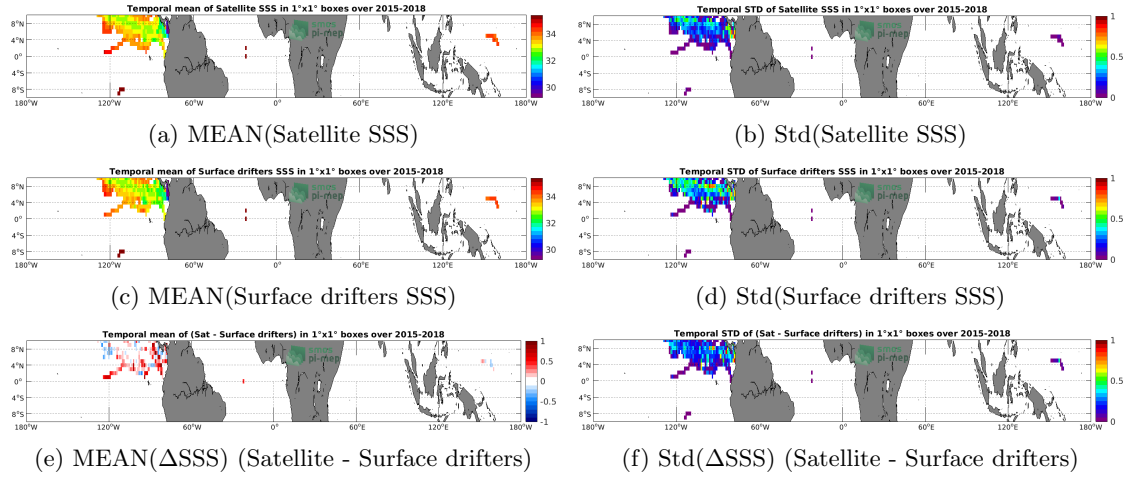
Figure 5: Temporal mean (left) and Std (right) of SSS from SMAP SSS L3 v4 - Monthly (RSS) (top), Surface drifters (middle), and of \Delta SSS (Satellite - Surface drifters). Only match-up pairs are used to generate these maps.
