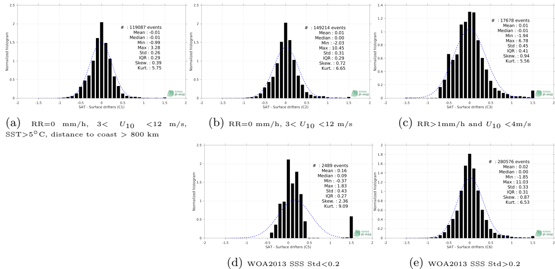
Figure 12: Normalized histogram of \Delta SSS (SMAP SSS L3 v4 - Monthly (RSS) - Surface drifters) for 5 different subdatasets corresponding to: RR=0 mm/h, 3 < U_{10} < 12 m/s, SST >5^\circ\text{C} , distance to coast > 800 km (a), RR=0 mm/h, 3 < U_{10} < 12 m/s (b), RR >1 mm/h and U_{10} < 4 m/s (c), WOA2013 SSS Std <0.2 (d), WOA2013 SSS Std >0.2 (e).
