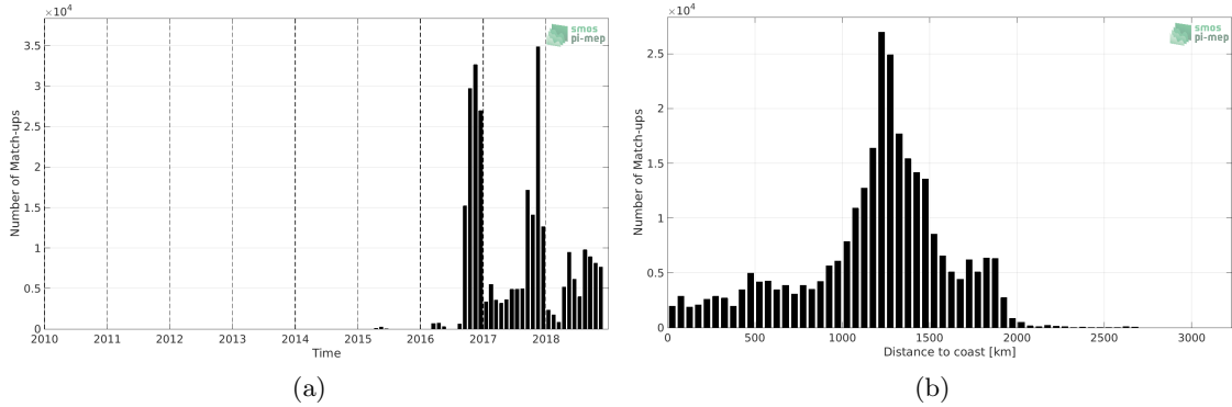
Figure 1: Number of match-ups between Surface drifters and SMAP SSS L3 v4 - Monthly (RSS) SSS as a function of time (a) and as function of the distance to coast (b) over the Equatorial Ocean 10N-10S Pi-MEP region and for the full satellite product period.
