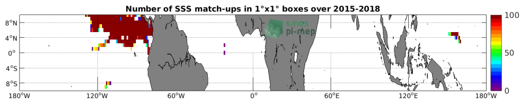
Figure 3: Number of SSS match-ups between Surface drifters SSS and the SMAP SSS L3 v4 - Monthly (RSS) SSS product for the Equatorial Ocean 10N-10S Pi-MEP region over 1^\circ \times 1^\circ boxes and for the full satellite product period.
