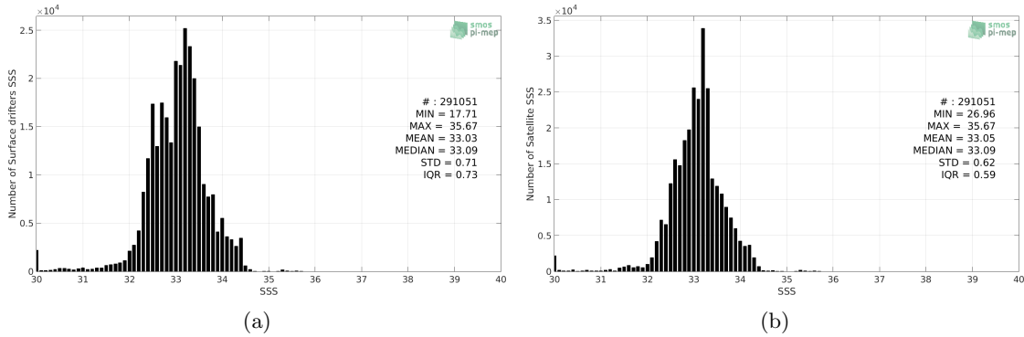
Figure 2: Histograms of SSS from Surface drifters (a) and SMAP-L3-RSS-V4-MONTHLY (b) considering all match-up pairs per bins of 0.1 over the Equatorial Ocean 10N-10S Pi-MEP region and for the full satellite product period.
