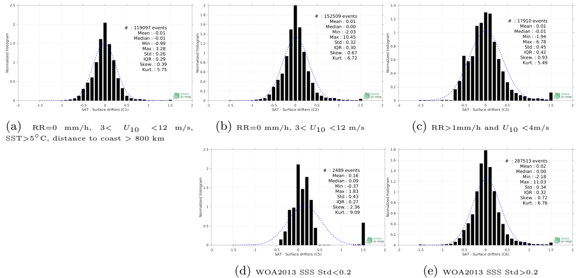
Figure 12: Normalized histogram of \Delta SSS (SMAP-L3-RSS-V4-MONTHLY - Surface drifters) for 5 different subdatasets corresponding to: RR=0 mm/h, 3 < U_{10} < 12 m/s, SST >5^\circ\text{C} , distance to coast > 800 km (a), RR=0 mm/h, 3 < U_{10} < 12 m/s (b), RR >1 mm/h and U_{10} < 4 m/s (c), WOA2013 SSS Std <0.2 (d), WOA2013 SSS Std >0.2 (e).
