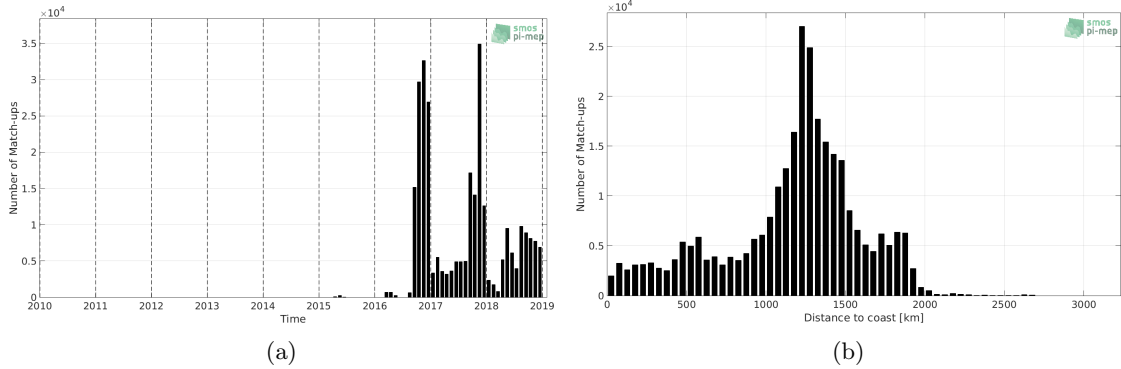
Figure 1: Number of match-ups between Surface drifters and SMAP-L3-RSS-V4-MONTHLY SSS as a function of time (a) and as function of the distance to coast (b) over the Equatorial Ocean 10N-10S Pi-MEP region and for the full satellite product period.
