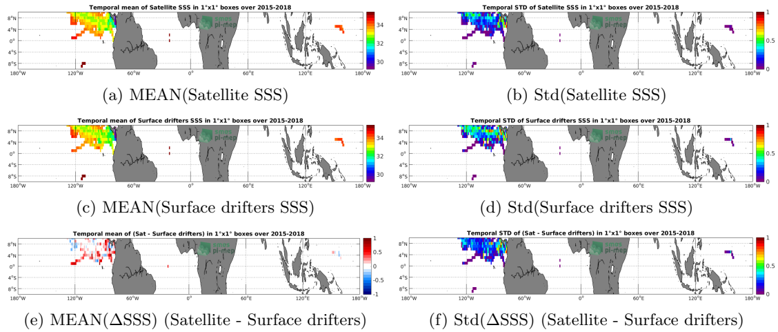
Figure 5: Temporal mean (left) and Std (right) of SSS from SMAP-L3-RSS-V4-MONTHLY (top), Surface drifters (middle), and of \Delta SSS (Satellite - Surface drifters). Only match-up pairs are used to generate these maps.
