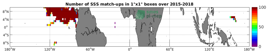
Figure 3: Number of SSS match-ups between Surface drifters SSS and the SMAP-L3-RSS-V4-MONTHLY SSS product for the Equatorial Ocean 10N-10S Pi-MEP region over 1^\circ \times 1^\circ boxes and for the full satellite product period.
