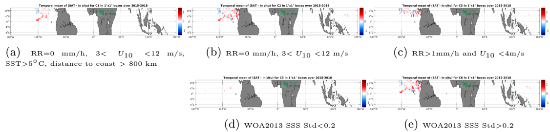
Figure 11: Temporal mean gridded over spatial boxes of size 1^\circ \times 1^\circ of \Delta SSS (SMAP-L3-RSS-V4-MONTHLY - Surface drifters) for 5 different subdatasets corresponding to:RR=0 mm/h, 3 < U_{10} < 12 m/s, SST >5^\circ\text{C} , distance to coast > 800 km (a), RR=0 mm/h, 3 < U_{10} < 12 m/s (b), RR >1 mm/h and U_{10} < 4 m/s (c), WOA2013 SSS Std <0.2 (d), WOA2013 SSS Std >0.2 (e).
