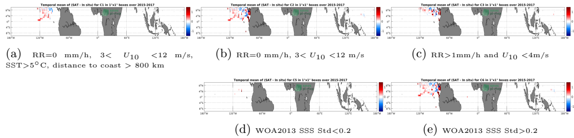
Figure 11: Temporal mean gridded over spatial boxes of size 1^\circ \times 1^\circ of \Delta SSS (SMAP-L3-RSS-V4-MONTHLY - Surface drifters) for 5 different subdatasets corresponding to: RR=0 mm/h, 3 < U_{10} < 12 m/s, SST >5^\circ C, distance to coast > 800 km (a), RR=0 mm/h, 3 < U_{10} < 12 m/s (b), RR >1 mm/h and U_{10} < 4 m/s (c), WOA2013 SSS Std <0.2 (d), WOA2013 SSS Std >0.2 (e).
