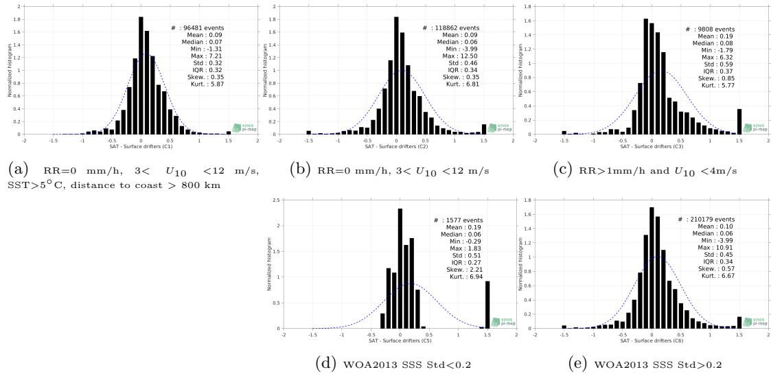
Figure 12: Normalized histogram of \Delta SSS (SMAP-L3-RSS-V4-MONTHLY - Surface drifters) for 5 different subdatasets corresponding to: RR=0 mm/h, 3 < U_{10} < 12 m/s, SST >5^\circ C, distance to coast > 800 km (a), RR=0 mm/h, 3 < U_{10} < 12 m/s (b), RR >1 mm/h and U_{10} < 4 m/s (c), WOA2013 SSS Std <0.2 (d), WOA2013 SSS Std >0.2 (e).
