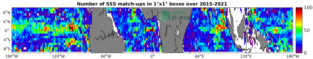
Figure 4: Number of SSS match-ups between Argo SSS and the SMAP SSS L3 v4 - Monthly (RSS) SSS product for the Equatorial Ocean 10N-10S Pi-MEP region over 1^\circ \times 1^\circ boxes and for the full satellite product period.
