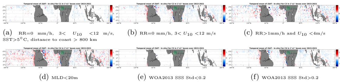
Figure 12: Temporal mean gridded over spatial boxes of size 1^\circ \times 1^\circ of \Delta SSS (SMAP SSS L3 v4 - Monthly (RSS) - Argo) for 6 different subdatasets corresponding to:RR=0 mm/h, 3 < U_{10} < 12 m/s, SST>5°C, distance to coast > 800 km (a), RR=0 mm/h, 3 < U_{10} < 12 m/s (b), RR>1mm/h and U_{10} < 4 m/s (c),MLD<20m (d),WOA2013 SSS Std<0.2 (e),WOA2013 SSS Std>0.2 (f).
