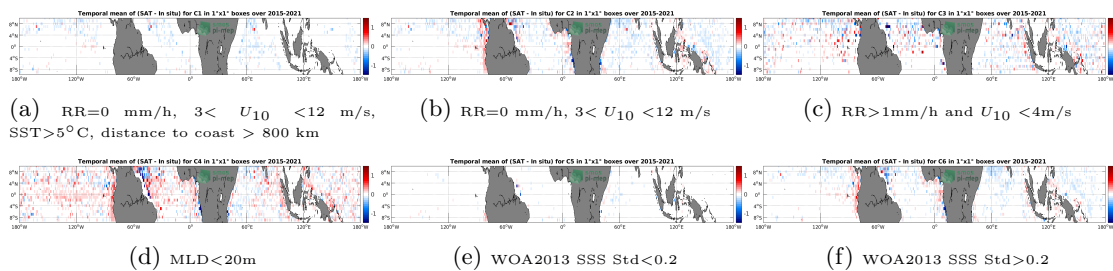
Figure 12: Temporal mean gridded over spatial boxes of size 1°x1° of \Delta SSS (SMAP SSS L3 v4 - Monthly (RSS) - Argo) for 6 different subdatasets corresponding to:RR=0 mm/h, 3 < U_{10} < 12 m/s, SST>5°C, distance to coast > 800 km (a), RR=0 mm/h, 3 < U_{10} < 12 m/s (b), RR>1mm/h and U_{10} < 4 m/s (c),MLD<20m (d),WOA2013 SSS Std<0.2 (e),WOA2013 SSS Std>0.2 (f).
