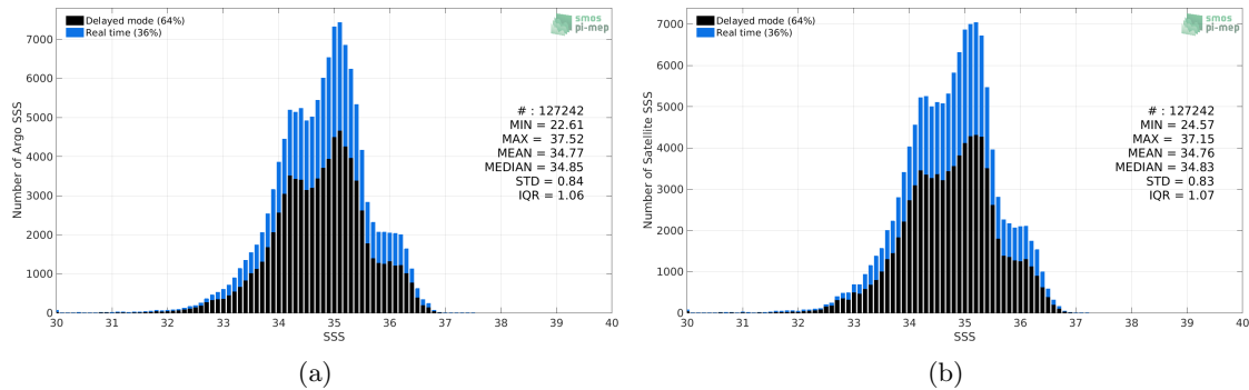
Figure 2: Histograms of SSS from Argo (a) and SMAP SSS L3 v4 - Monthly (RSS) (b) considering all match-up pairs per bins of 0.1 over the Equatorial Ocean 10N-10S Pi-MEP region and for the full satellite product period.
