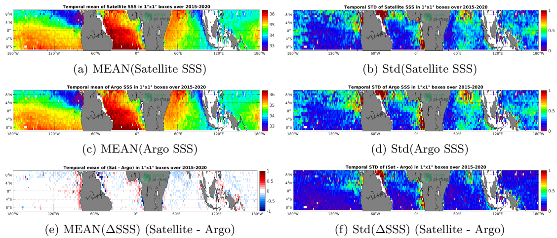
Figure 6: Temporal mean (left) and Std (right) of SSS from SMAP SSS L3 v4 - Monthly (RSS) (top), Argo (middle), and of \Delta SSS (Satellite - Argo). Only match-up pairs are used to generate these maps.
