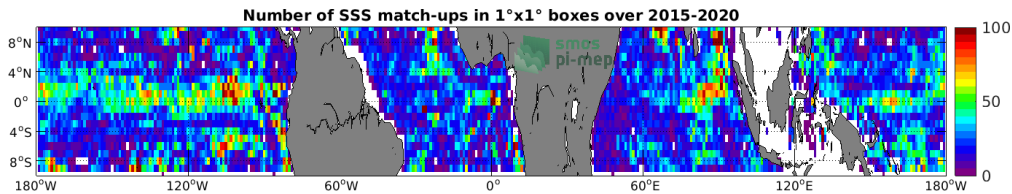
Figure 4: Number of SSS match-ups between Argo SSS and the SMAP SSS L3 v4 - Monthly (RSS) SSS product for the Equatorial Ocean 10N-10S Pi-MEP region over 1°x1° boxes and for the full satellite product period.
