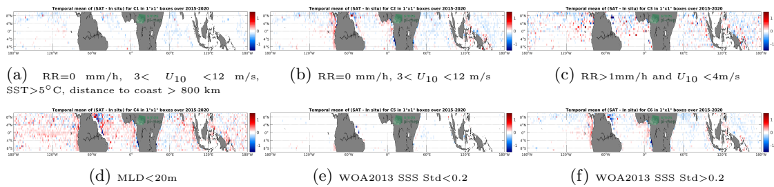
Figure 12: Temporal mean gridded over spatial boxes of size 1°x1° of ΔSSS (SMAP SSS L3 v4 - Monthly (RSS) - Argo) for 6 different subdatasets corresponding to:RR=0 mm/h, 3 < U 10 <12 m/s, SST>5°C, distance to coast > 800 km (a), RR=0 mm/h, 3 < U 10 <12 m/s (b), RR>1mm/h and U 10 <4m/s (c),MLD<20m (d),WOA2013 SSS Std<0.2 (e),WOA2013 SSS Std>0.2 (f).
