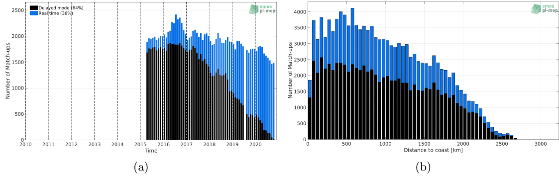
Figure 1: Number of match-ups between Argo and SMAP SSS L3 v4 - Monthly (RSS) SSS as a function of time (a) and as function of the distance to coast (b) over the Equatorial Ocean 10N-10S Pi-MEP region and for the full satellite product period.
