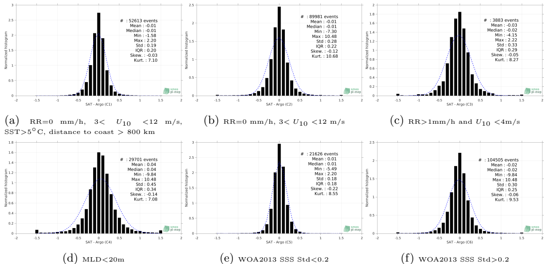
Figure 13: Normalized histogram of ΔSSS (SMAP SSS L3 v4 - Monthly (RSS) - Argo) for 6 different subdatasets corresponding to: RR=0 mm/h, 3 < U 10 <12 m/s, SST>5°C, distance to coast > 800 km (a), RR=0 mm/h, 3 < U 10 <12 m/s (b), RR>1mm/h and U 10 <4m/s (c), MLD<20m (d), WOA2013 SSS Std<0.2 (e), WOA2013 SSS Std>0.2 (f).
