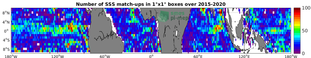
Figure 4: Number of SSS match-ups between Argo SSS and the SMAP-L3-RSS-V4-MONTHLY SSS product for the Equatorial Ocean 10N-10S Pi-MEP region over 1^\circ \times 1^\circ boxes and for the full satellite product period.
