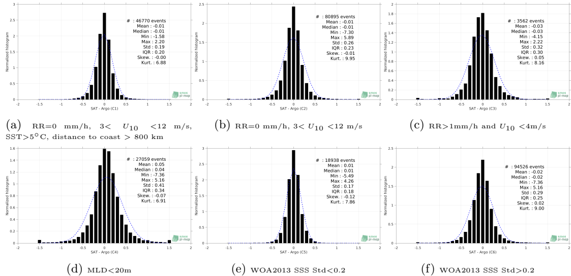
Figure 13: Normalized histogram of \Delta SSS (SMAP-L3-RSS-V4-MONTHLY - Argo) for 6 different subdatasets corresponding to: RR=0 mm/h, 3 < U_{10} < 12 m/s, SST >5^\circ C, distance to coast > 800 km (a), RR=0 mm/h, 3 < U_{10} < 12 m/s (b), RR >1 mm/h and U_{10} < 4 m/s (c), MLD <20 m (d), WOA2013 SSS Std <0.2 (e), WOA2013 SSS Std >0.2 (f).
