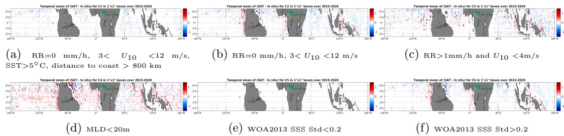
Figure 12: Temporal mean gridded over spatial boxes of size 1^\circ \times 1^\circ of \Delta SSS (SMAP-L3-RSS-V4-MONTHLY - Argo) for 6 different subdatasets corresponding to:RR=0 mm/h, 3 < U_{10} < 12 m/s, SST >5^\circ C, distance to coast > 800 km (a), RR=0 mm/h, 3 < U_{10} < 12 m/s (b), RR >1 mm/h and U_{10} < 4 m/s (c),MLD <20 m (d),WOA2013 SSS Std <0.2 (e),WOA2013 SSS Std >0.2 (f).
