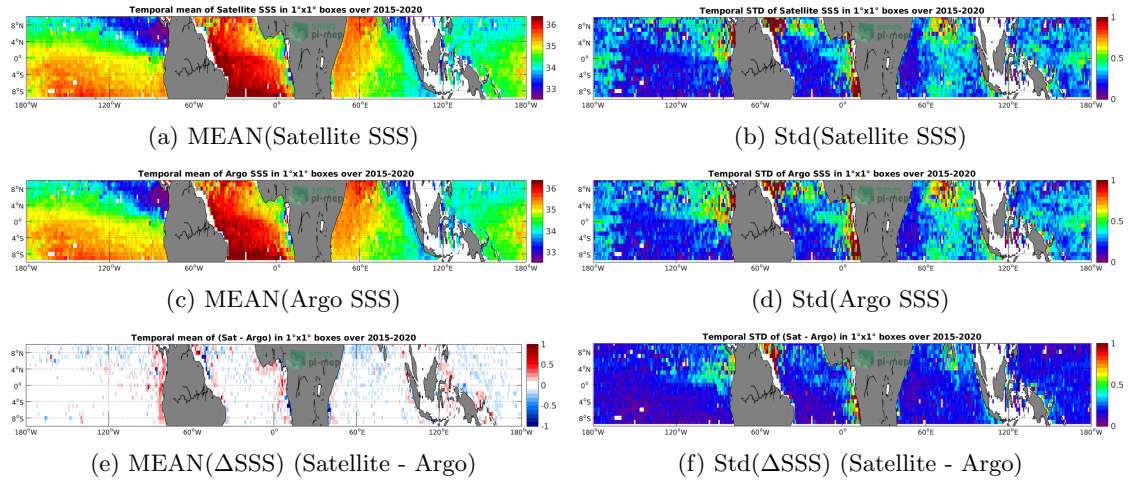
Figure 6: Temporal mean (left) and Std (right) of SSS from SMAP-L3-RSS-V4-MONTHLY (top), Argo (middle), and of \Delta SSS (Satellite - Argo). Only match-up pairs are used to generate these maps.
