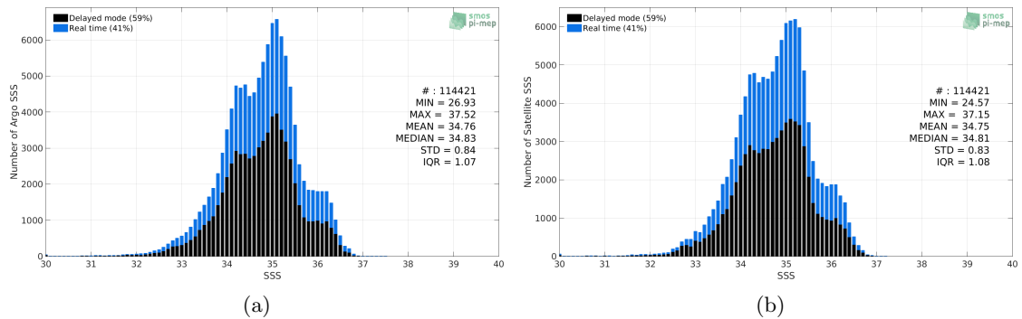
Figure 2: Histograms of SSS from Argo (a) and SMAP-L3-RSS-V4-MONTHLY (b) considering all match-up pairs per bins of 0.1 over the Equatorial Ocean 10N-10S Pi-MEP region and for the full satellite product period.
