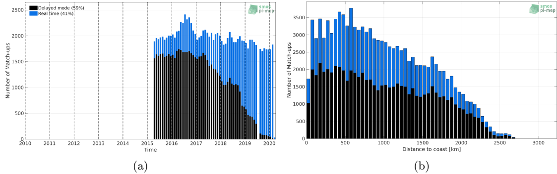
Figure 1: Number of match-ups between Argo and SMAP-L3-RSS-V4-MONTHLY SSS as a function of time (a) and as function of the distance to coast (b) over the Equatorial Ocean 10N-10S Pi-MEP region and for the full satellite product period.
