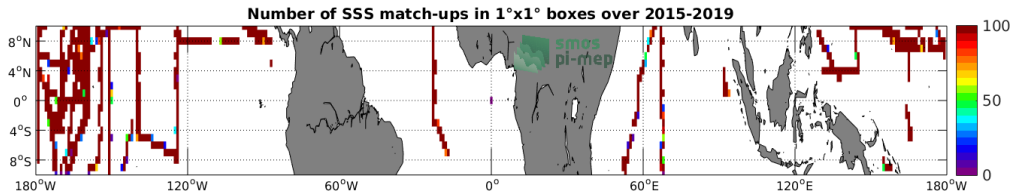
Figure 4: Number of SSS match-ups between TSG-SAMOS SSS and the SMAP-L3-RSS-V3-8DAY-RUNNING-70KM SSS product for the Equatorial Ocean 10N-10S Pi-MEP region over 1°x1° boxes and for the full satellite product period.
