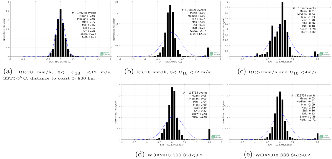
Figure 13: Normalized histogram of \Delta SSS (SMAP-L3-RSS-V3-8DAY-RUNNING-70KM - TSG-SAMOS) for 5 different subdatasets corresponding to: RR=0 mm/h, 3 < U_{10} < 12 m/s, SST > 5^\circ C , distance to coast > 800 km (a), RR=0 mm/h, 3 < U_{10} < 12 m/s (b), RR > 1 mm/h and U_{10} < 4 m/s (c), WOA2013 SSS Std < 0.2 (d), WOA2013 SSS Std > 0.2 (e).
