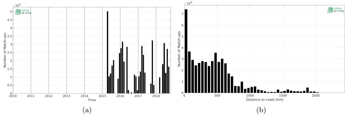
Figure 1: Number of match-ups between TSG-SAMOS and SMAP-L3-RSS-V3-8DAY-RUNNING-70KM SSS as a function of time (a) and as function of the distance to coast (b) over the Equatorial Ocean 10N-10S Pi-MEP region and for the full satellite product period.
