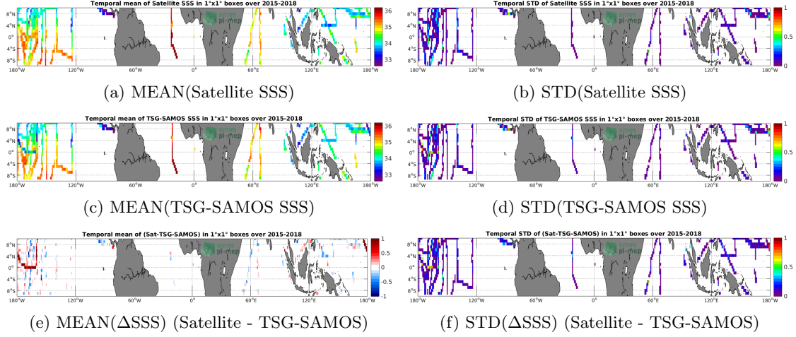
Figure 6: Temporal mean (left) and STD (right) of SSS from SMAP-L3-RSS-V3-8DAY-RUNNING-70KM (top), TSG-SAMOS (middle), and of \Delta SSS (Satellite - TSG-SAMOS). Only match-up pairs are used to generate these maps.
