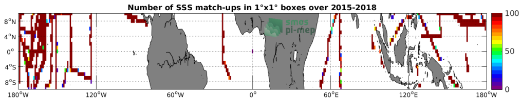
Figure 4: Number of SSS match-ups between TSG-SAMOS SSS and the SMAP-L3-RSS-V3-8DAY-RUNNING-70KM SSS product for the Equatorial Ocean 10N-10S Pi-MEP region over 1^\circ \times 1^\circ boxes and for the full satellite product period.
