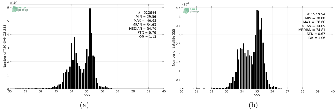
Figure 2: Histograms of SSS from TSG-SAMOS (a) and SMAP-L3-RSS-V3-8DAY-RUNNING-70KM (b) considering all match-up pairs per bins of 0.1 over the Equatorial Ocean 10N-10S Pi-MEP region and for the full satellite product period.
