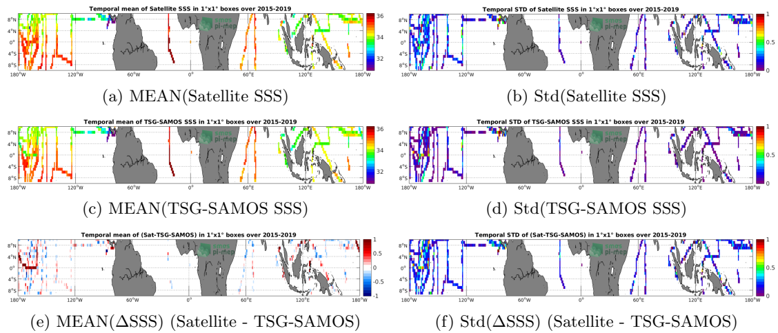
Figure 6: Temporal mean (left) and Std (right) of SSS from SMAP-L3-RSS-V3-8DAY-RUNNING-40KM (top), TSG-SAMOS (middle), and of \Delta SSS (Satellite - TSG-SAMOS). Only match-up pairs are used to generate these maps.
