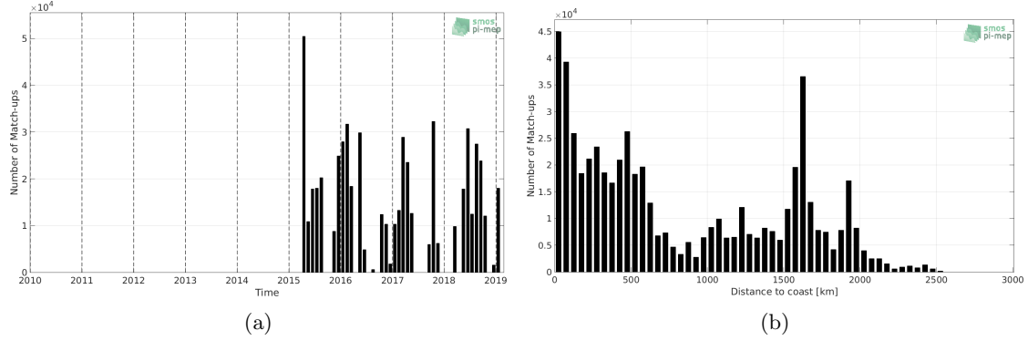
Figure 1: Number of match-ups between TSG-SAMOS and SMAP-L3-RSS-V3-8DAY-RUNNING-40KM SSS as a function of time (a) and as function of the distance to coast (b) over the Equatorial Ocean 10N-10S Pi-MEP region and for the full satellite product period.
