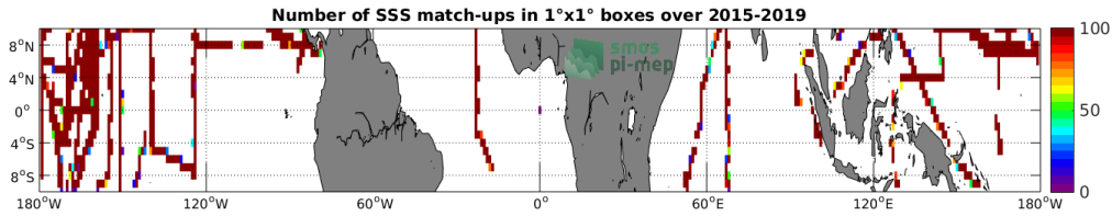
Figure 4: Number of SSS match-ups between TSG-SAMOS SSS and the SMAP-L3-RSS-V3-8DAY-RUNNING-40KM SSS product for the Equatorial Ocean 10N-10S Pi-MEP region over 1°x1° boxes and for the full satellite product period.
