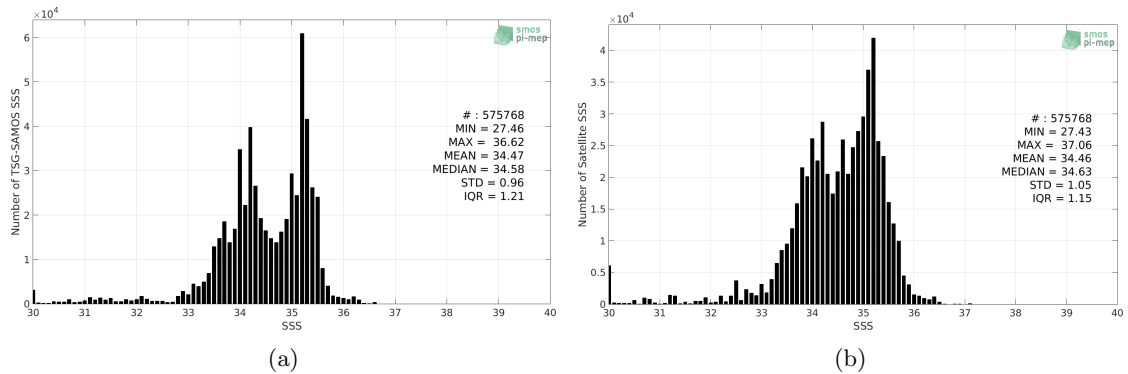
Figure 2: Histograms of SSS from TSG-SAMOS (a) and SMAP-L3-RSS-V3-8DAY-RUNNING-40KM (b) considering all match-up pairs per bins of 0.1 over the Equatorial Ocean 10N-10S Pi-MEP region and for the full satellite product period.
