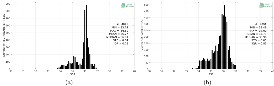
Figure 2: Histograms of SSS from TSG-POLARSTERN (a) and SMAP-L3-RSS-V3-8DAY-RUNNING-40KM (b) considering all match-up pairs per bins of 0.1 over the Equatorial Ocean 10N-10S Pi-MEP region and for the full satellite product period.
