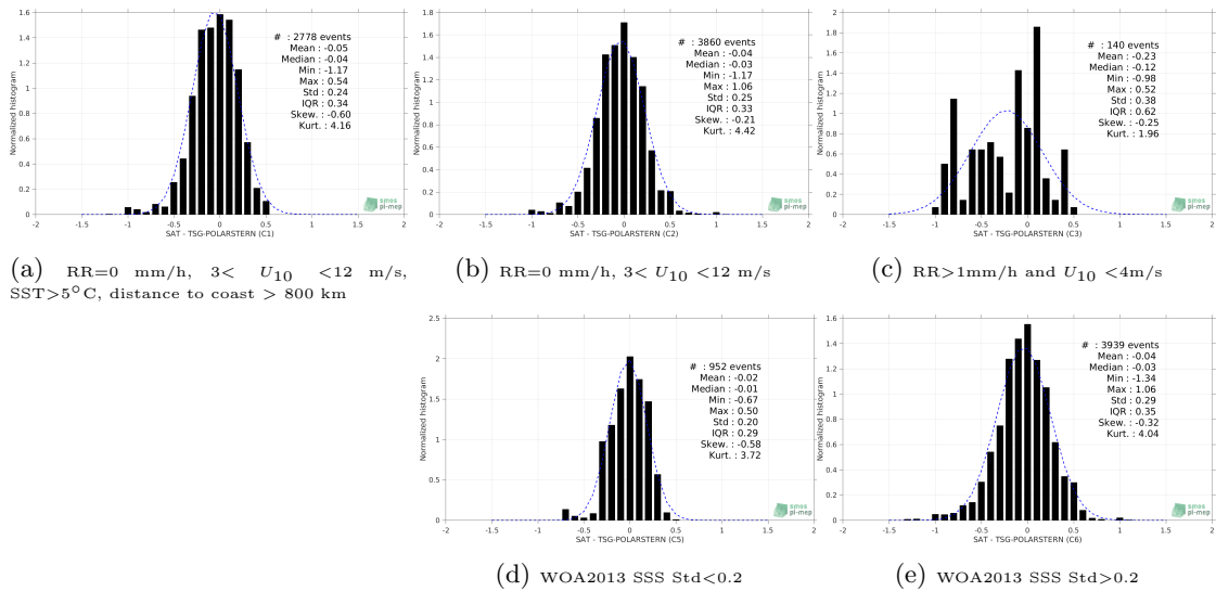
Figure 13: Normalized histogram of \Delta SSS (SMAP-L3-RSS-V3-8DAY-RUNNING-40KM - TSG-POLARSTERN) for 5 different subdatasets corresponding to: RR=0 mm/h, 3 < U_{10} < 12 m/s, SST >5^\circ C, distance to coast > 800 km (a), RR=0 mm/h, 3 < U_{10} < 12 m/s (b), RR >1 mm/h and U_{10} < 4 m/s (c), WOA2013 SSS Std <0.2 (d), WOA2013 SSS Std >0.2 (e).
