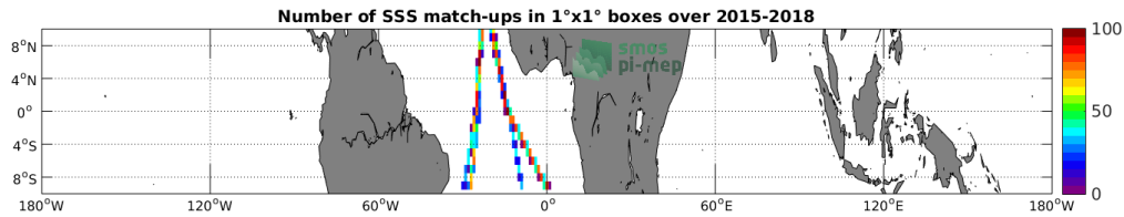
Figure 4: Number of SSS match-ups between TSG-POLARSTERN SSS and the SMAP-L3-RSS-V3-8DAY-RUNNING-40KM SSS product for the Equatorial Ocean 10N-10S Pi-MEP region over 1^\circ \times 1^\circ boxes and for the full satellite product period.
