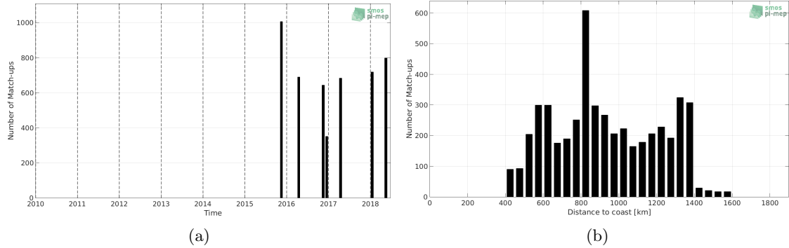
Figure 1: Number of match-ups between TSG-POLARSTERN and SMAP-L3-RSS-V3-8DAY-RUNNING-40KM SSS as a function of time (a) and as function of the distance to coast (b) over the Equatorial Ocean 10N-10S Pi-MEP region and for the full satellite product period.
