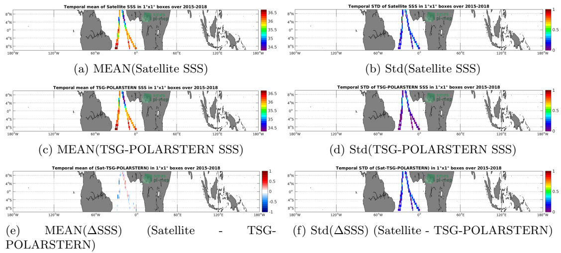
Figure 6: Temporal mean (left) and Std (right) of SSS from SMAP-L3-RSS-V3-8DAY-RUNNING-40KM (top), TSG-POLARSTERN (middle), and of \Delta SSS (Satellite - TSG-POLARSTERN). Only match-up pairs are used to generate these maps.
