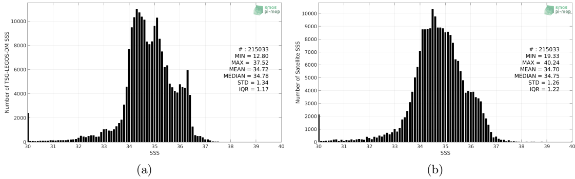
Figure 2: Histograms of SSS from TSG-LEGOS-DM (a) and SMAP-L3-RSS-V3-8DAY-RUNNING-40KM (b) considering all match-up pairs per bins of 0.1 over the Equatorial Ocean 10N-10S Pi-MEP region and for the full satellite product period.
