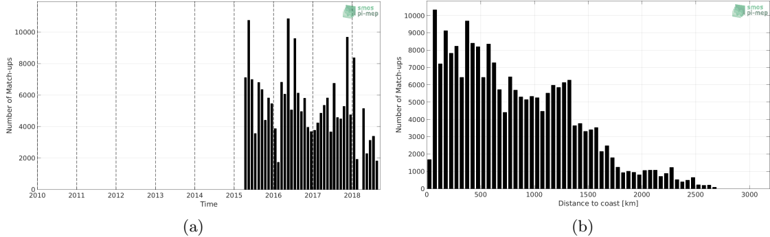
Figure 1: Number of match-ups between TSG-LEGOS-DM and SMAP-L3-RSS-V3-8DAY-RUNNING-40KM SSS as a function of time (a) and as function of the distance to coast (b) over the Equatorial Ocean 10N-10S Pi-MEP region and for the full satellite product period.
