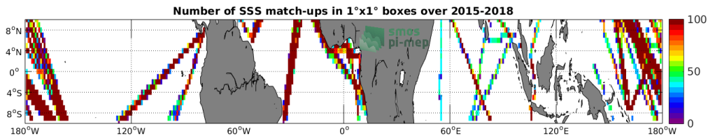
Figure 4: Number of SSS match-ups between TSG-LEGOS-DM SSS and the SMAP-L3-RSS-V3-8DAY-RUNNING-40KM SSS product for the Equatorial Ocean 10N-10S Pi-MEP region over 1^\circ \times 1^\circ boxes and for the full satellite product period.
