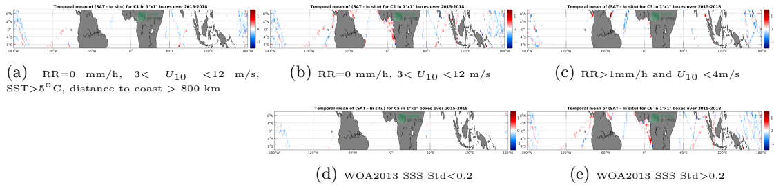
Figure 12: Temporal mean gridded over spatial boxes of size 1^\circ \times 1^\circ of \Delta SSS (SMAP-L3-RSS-V3-8DAY-RUNNING-40KM - TSG-LEGOS-DM) for 5 different subdatasets corresponding to:RR=0 mm/h, 3 < U_{10} < 12 m/s, SST >5^\circ C, distance to coast > 800 km (a), RR=0 mm/h, 3 < U_{10} < 12 m/s (b), RR >1 mm/h and U_{10} < 4 m/s (c), WOA2013 SSS Std <0.2 (d), WOA2013 SSS Std >0.2 (e).
