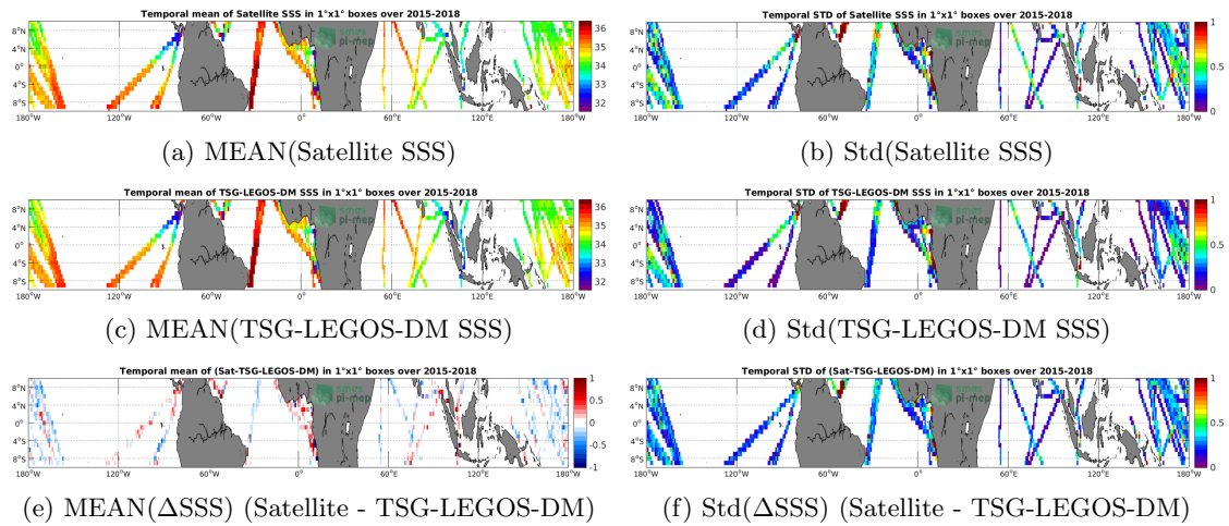
Figure 6: Temporal mean (left) and Std (right) of SSS from SMAP-L3-RSS-V3-8DAY-RUNNING-40KM (top), TSG-LEGOS-DM (middle), and of \Delta SSS (Satellite - TSG-LEGOS-DM). Only match-up pairs are used to generate these maps.
