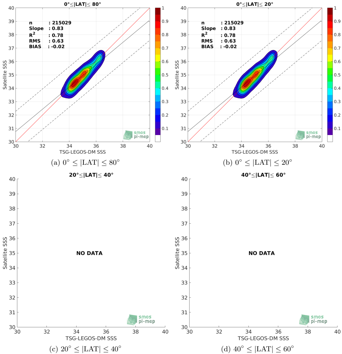
Figure 9: Contour maps of the concentration of SMAP-L3-RSS-V3-8DAY-RUNNING-40KM SSS (y-axis) versus TSG-LEGOS-DM SSS (x-axis) at match-up pairs for different latitude bands. For each plot, the red line shows x=y . The black thin and dashed lines indicate a linear fit through the data cloud and the \pm 95\% confidence levels, respectively. The number match-up pairs n , the slope and R^2 coefficient of the linear fit, the root mean square (RMS) and the mean bias between satellite and in situ data are indicated for each latitude band in each plots.
