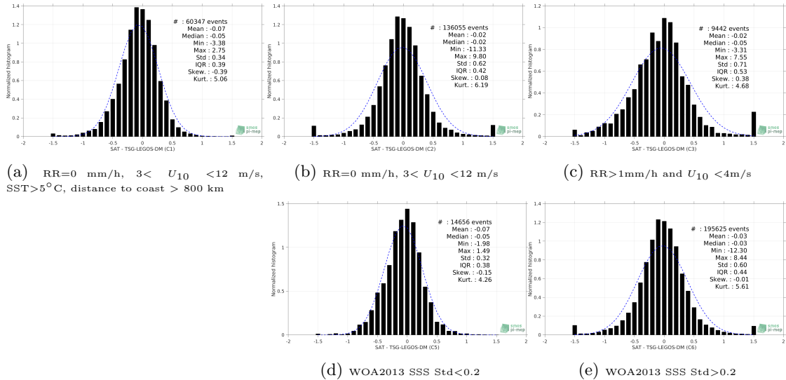
Figure 13: Normalized histogram of \Delta SSS (SMAP-L3-RSS-V3-8DAY-RUNNING-40KM - TSG-LEGOS-DM) for 5 different subdatasets corresponding to: RR=0 mm/h, 3 < U_{10} < 12 m/s, SST >5^\circ C, distance to coast > 800 km (a), RR=0 mm/h, 3 < U_{10} < 12 m/s (b), RR >1 mm/h and U_{10} < 4 m/s (c), WOA2013 SSS Std <0.2 (d), WOA2013 SSS Std >0.2 (e).
