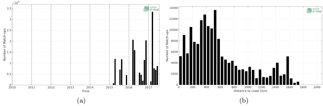
Figure 1: Number of match-ups between TSG-GOSUD-Research-vessel and SMAP-L3-RSS-V3-8DAY-RUNNING-40KM SSS as a function of time (a) and as function of the distance to coast (b) over the Equatorial Ocean 10N-10S Pi-MEP region and for the full satellite product period.
