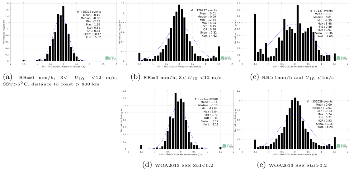
Figure 13: Normalized histogram of \Delta SSS (SMAP-L3-RSS-V3-8DAY-RUNNING-40KM - TSG-GOSUD-Research-vessel) for 5 different subdatasets corresponding to: RR=0 mm/h, 3 < U_{10} < 12 m/s, SST >5^\circ\text{C} , distance to coast > 800 km (a), RR=0 mm/h, 3 < U_{10} < 12 m/s (b), RR >1 mm/h and U_{10} < 4 m/s (c), WOA2013 SSS Std <0.2 (d), WOA2013 SSS Std >0.2 (e).
