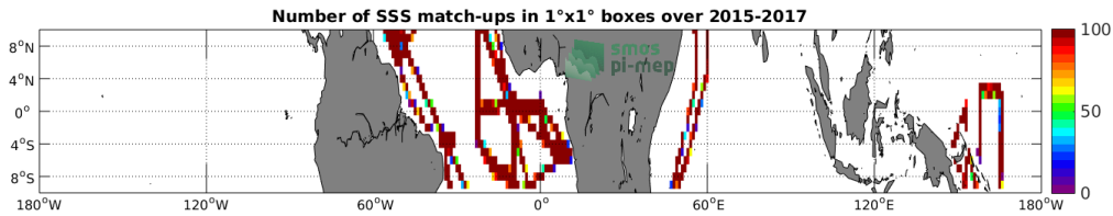
Figure 4: Number of SSS match-ups between TSG-GOSUD-Research-vessel SSS and the SMAP-L3-RSS-V3-8DAY-RUNNING-40KM SSS product for the Equatorial Ocean 10N-10S Pi-MEP region over 1^\circ \times 1^\circ boxes and for the full satellite product period.
