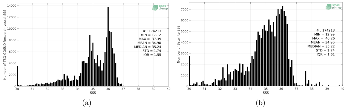
Figure 2: Histograms of SSS from TSG-GOSUD-Research-vessel (a) and SMAP-L3-RSS-V3-8DAY-RUNNING-40KM (b) considering all match-up pairs per bins of 0.1 over the Equatorial Ocean 10N-10S Pi-MEP region and for the full satellite product period.
