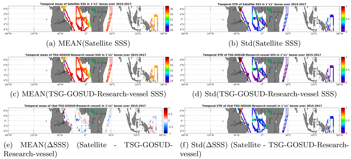
Figure 6: Temporal mean (left) and Std (right) of SSS from SMAP-L3-RSS-V3-8DAY-RUNNING-40KM (top), TSG-GOSUD-Research-vessel (middle), and of \Delta SSS (Satellite - TSG-GOSUD-Research-vessel). Only match-up pairs are used to generate these maps.
