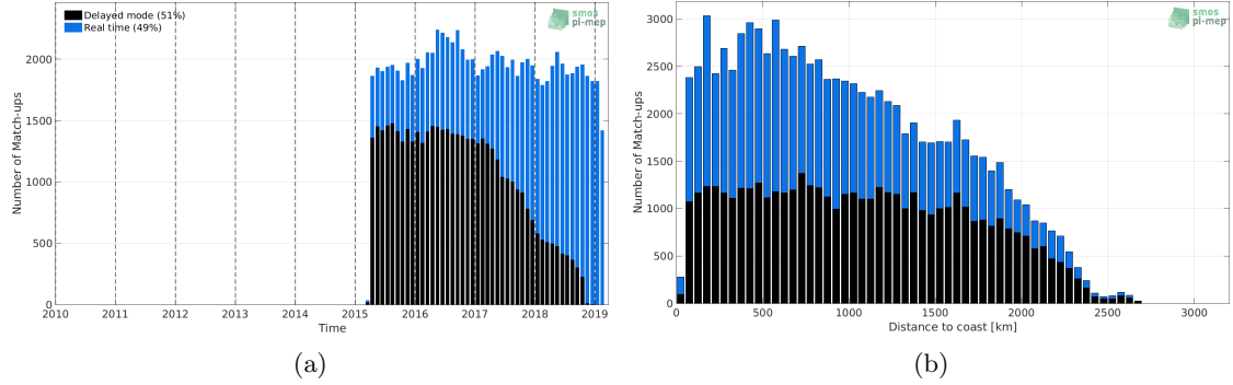
Figure 1: Number of match-ups between Argo and SMAP-L3-RSS-V3-8DAY-RUNNING-40KM SSS as a function of time (a) and as function of the distance to coast (b) over the Equatorial Ocean 10N-10S Pi-MEP region and for the full satellite product period.
