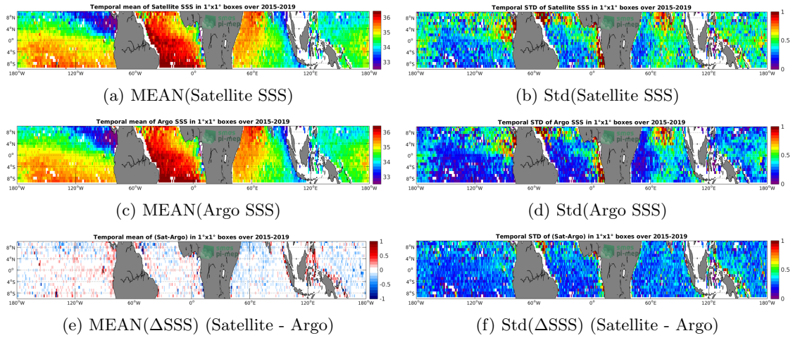
Figure 6: Temporal mean (left) and Std (right) of SSS from SMAP-L3-RSS-V3-8DAY-RUNNING-40KM (top), Argo (middle), and of \Delta SSS (Satellite - Argo). Only match-up pairs are used to generate these maps.
