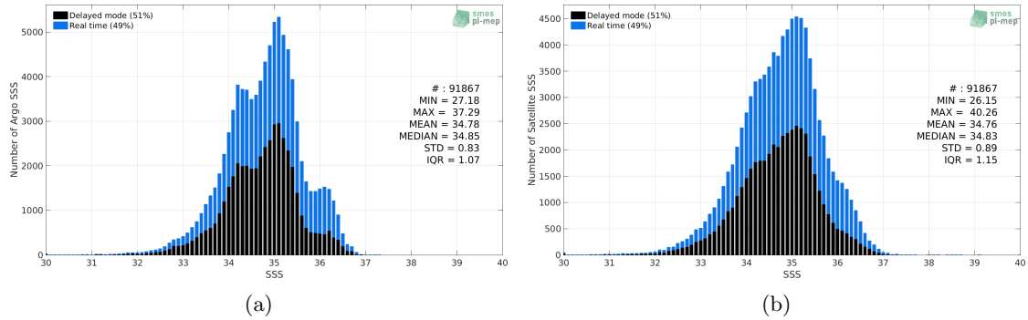
Figure 2: Histograms of SSS from Argo (a) and SMAP-L3-RSS-V3-8DAY-RUNNING-40KM (b) considering all match-up pairs per bins of 0.1 over the Equatorial Ocean 10N-10S Pi-MEP region and for the full satellite product period.
