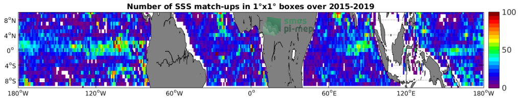
Figure 4: Number of SSS match-ups between Argo SSS and the SMAP-L3-RSS-V3-8DAY-RUNNING-40KM SSS product for the Equatorial Ocean 10N-10S Pi-MEP region over 1^\circ \times 1^\circ boxes and for the full satellite product period.
