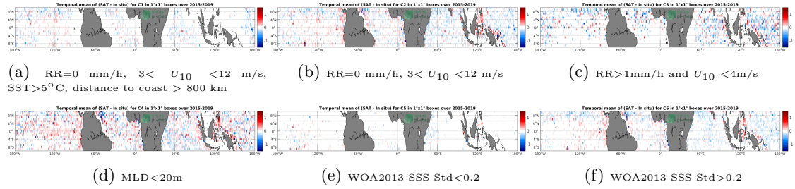
Figure 12: Temporal mean gridded over spatial boxes of size 1^\circ \times 1^\circ of \Delta SSS (SMAP-L3-RSS-V3-8DAY-RUNNING-40KM - Argo) for 6 different subdatasets corresponding to: RR=0 mm/h, 3 < U_{10} < 12 m/s, SST > 5^\circ C , distance to coast > 800 km (a), RR=0 mm/h, 3 < U_{10} < 12 m/s (b), RR > 1 mm/h and U_{10} < 4 m/s (c), MLD < 20 m (d), WOA2013 SSS Std < 0.2 (e), WOA2013 SSS Std > 0.2 (f).
