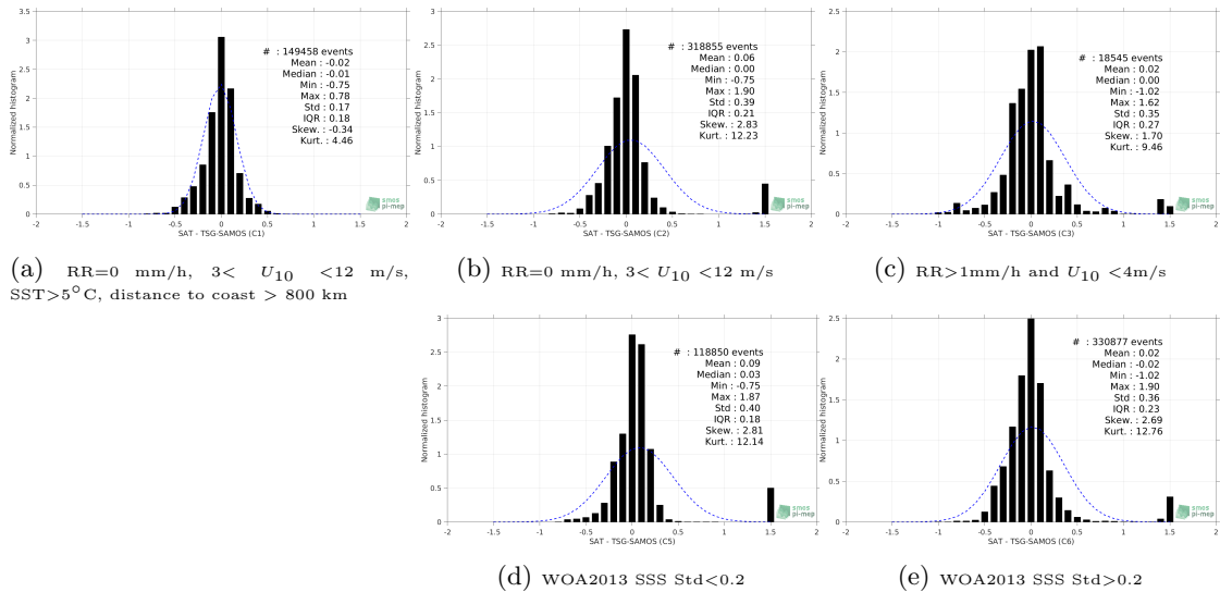
Figure 13: Normalized histogram of \Delta SSS (SMAP-L3-RSS-V3-MONTHLY-70KM - TSG-SAMOS) for 5 different subdatasets corresponding to: RR=0 mm/h, 3 < U_{10} < 12 m/s, SST > 5^\circ C , distance to coast > 800 km (a), RR=0 mm/h, 3 < U_{10} < 12 m/s (b), RR > 1 mm/h and U_{10} < 4 m/s (c), WOA2013 SSS Std < 0.2 (d), WOA2013 SSS Std > 0.2 (e).
