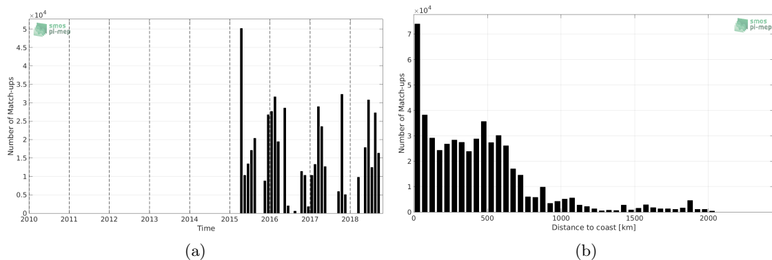
Figure 1: Number of match-ups between TSG-SAMOS and SMAP-L3-RSS-V3-MONTHLY-70KM SSS as a function of time (a) and as function of the distance to coast (b) over the Equatorial Ocean 10N-10S Pi-MEP region and for the full satellite product period.
