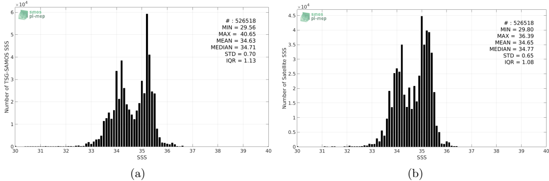
Figure 2: Histograms of SSS from TSG-SAMOS (a) and SMAP-L3-RSS-V3-MONTHLY-70KM (b) considering all match-up pairs per bins of 0.1 over the Equatorial Ocean 10N-10S Pi-MEP region and for the full satellite product period.
