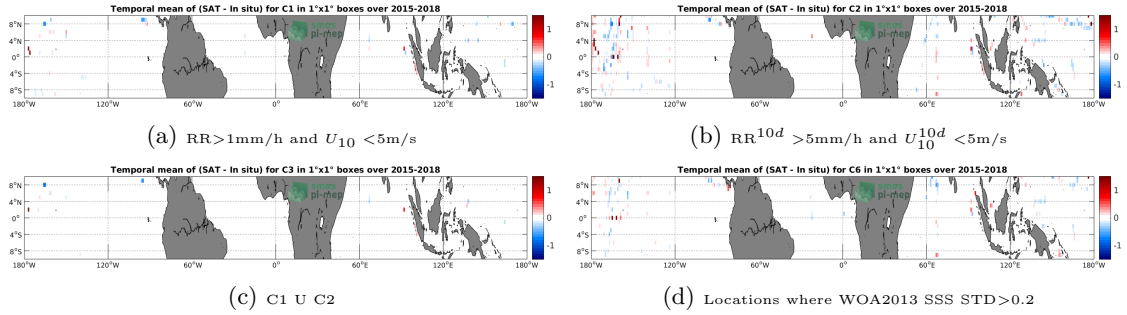
Figure 12: Temporal mean gridded over spatial boxes of size 1^\circ \times 1^\circ of \Delta SSS (SMAP-L3-RSS-V3-MONTHLY-70KM - TSG-SAMOS) for 4 different subdatasets corresponding to: RR > 1 mm/h and U_{10} < 5 m/s (a), RR 10d > 5 mm/h and U_{10}^{10d} < 5 m/s (b), C1 U C2 (c), Locations where WOA2013 SSS STD > 0.2 (d).
