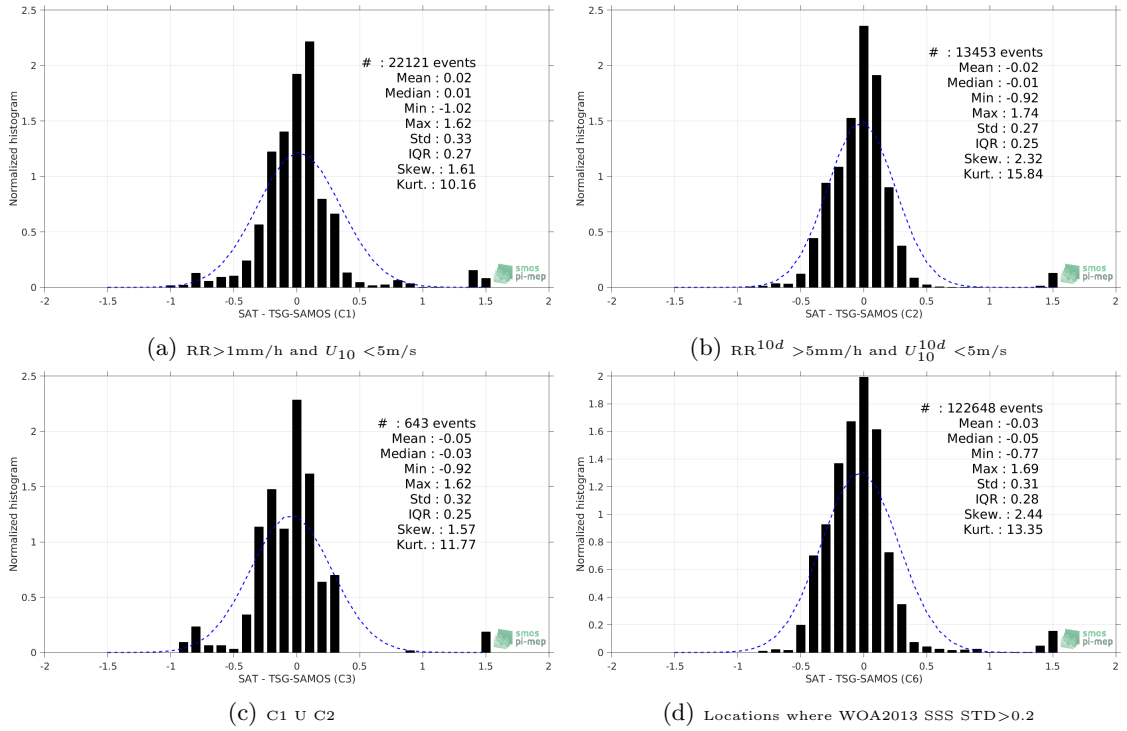
Figure 13: Normalized histogram of \Delta SSS (SMAP-L3-RSS-V3-MONTHLY-70KM - TSG-SAMOS) for 6 different subdatasets corresponding to: RR > 1 mm/h and U_{10} < 5 m/s (a), RR 10d > 5 mm/h and U_{10}^{10d} < 5 m/s (b), C1 U C2 (c), Locations where WOA2013 SSS STD > 0.2 (d).
