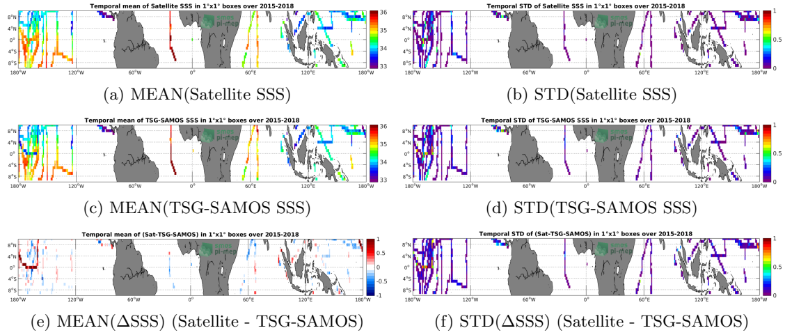
Figure 6: Temporal mean (left) and STD (right) of SSS from SMAP-L3-RSS-V3-MONTHLY-70KM (top), TSG-SAMOS (middle), and of \Delta SSS (Satellite - TSG-SAMOS). Only match-up pairs are used to generate these maps.
