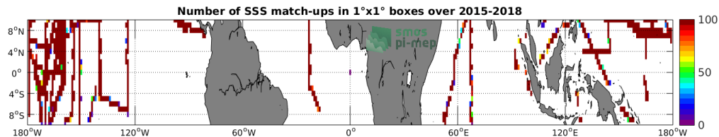
Figure 4: Number of SSS match-ups between TSG-SAMOS SSS and the SMAP-L3-RSS-V3-MONTHLY-70KM SSS product for the Equatorial Ocean 10N-10S Pi-MEP region over 1°x1° boxes and for the full satellite product period.
