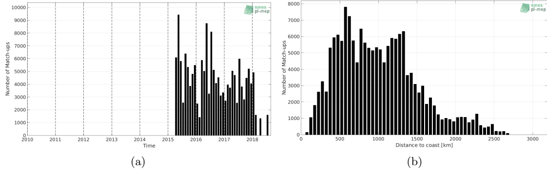
Figure 1: Number of match-ups between TSG-LEGOS-DM and SMAP-L3-RSS-V3-MONTHLY-70KM SSS as a function of time (a) and as function of the distance to coast (b) over the Equatorial Ocean 10N-10S Pi-MEP region and for the full satellite product period.
