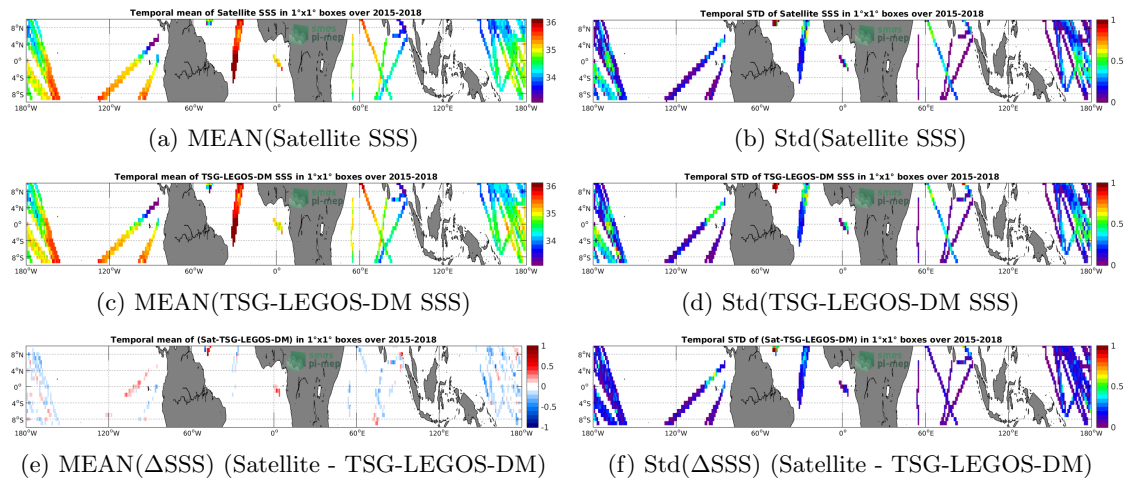
Figure 6: Temporal mean (left) and Std (right) of SSS from SMAP-L3-RSS-V3-MONTHLY-70KM (top), TSG-LEGOS-DM (middle), and of \Delta SSS (Satellite - TSG-LEGOS-DM). Only match-up pairs are used to generate these maps.
