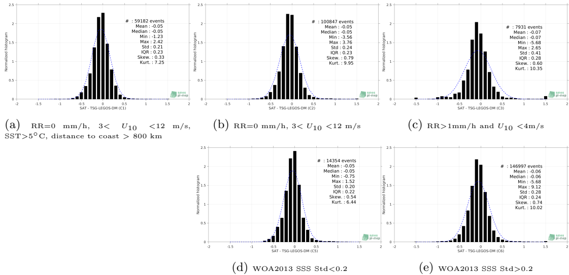
Figure 13: Normalized histogram of \Delta SSS (SMAP-L3-RSS-V3-MONTHLY-70KM - TSG-LEGOS-DM) for 5 different subdatasets corresponding to: RR=0 mm/h, 3 < U_{10} < 12 m/s, SST >5^\circ C, distance to coast > 800 km (a), RR=0 mm/h, 3 < U_{10} < 12 m/s (b), RR >1 mm/h and U_{10} < 4 m/s (c), WOA2013 SSS Std <0.2 (d), WOA2013 SSS Std >0.2 (e).
