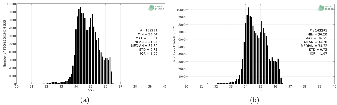
Figure 2: Histograms of SSS from TSG-LEGOS-DM (a) and SMAP-L3-RSS-V3-MONTHLY-70KM (b) considering all match-up pairs per bins of 0.1 over the Equatorial Ocean 10N-10S Pi-MEP region and for the full satellite product period.
