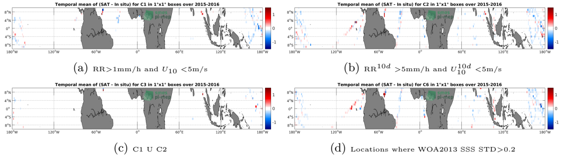
Figure 12: Temporal mean gridded over spatial boxes of size 1^\circ \times 1^\circ of \Delta SSS (SMAP-L3-RSS-V3-MONTHLY-70KM - TSG-LEGOS-DM) for 4 different subdatasets corresponding to: RR > 1\text{mm/h} and U_{10} < 5\text{m/s} (a), RR^{10d} > 5\text{mm/h} and U_{10}^{10d} < 5\text{m/s} (b), C1 U C2 (c), Locations where WOA2013 SSS STD > 0.2 (d).
