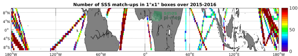
Figure 4: Number of SSS match-ups between TSG-LEGOS-DM SSS and the SMAP-L3-RSS-V3-MONTHLY-70KM SSS product for the Equatorial Ocean 10N-10S Pi-MEP region over 1^\circ \times 1^\circ boxes and for the full satellite product period.
