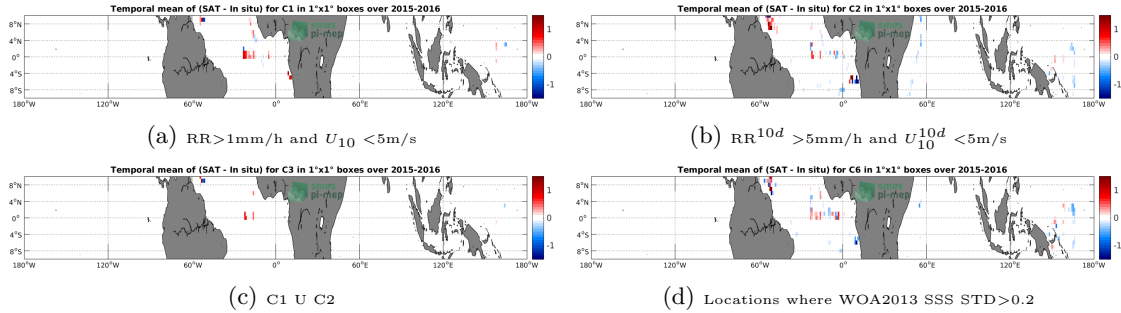
Figure 12: Temporal mean gridded over spatial boxes of size 1^\circ \times 1^\circ of \Delta SSS (SMAP-L3-RSS-V3-MONTHLY-70KM - TSG-GOSUD-Research-vessel) for 4 different subdatasets corresponding to: RR>1mm/h and U_{10} < 5\text{m/s} (a), RR^{10d} > 5\text{mm/h} and U_{10}^{10d} < 5\text{m/s} (b), C1 U C2 (c), Locations where WOA2013 SSS STD>0.2 (d).
