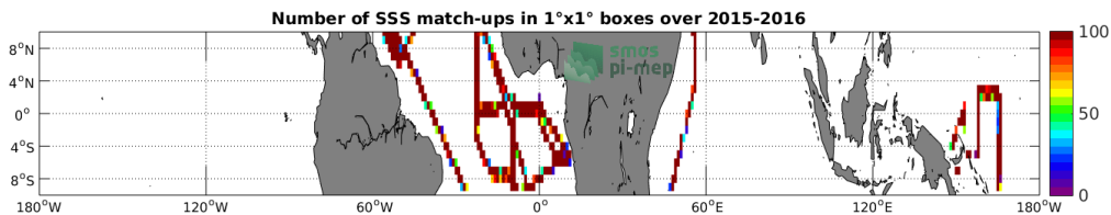
Figure 4: Number of SSS match-ups between TSG-GOSUD-Research-vessel SSS and the SMAP-L3-RSS-V3-MONTHLY-70KM SSS product for the Equatorial Ocean 10N-10S Pi-MEP region over 1^\circ \times 1^\circ boxes and for the full satellite product period.
