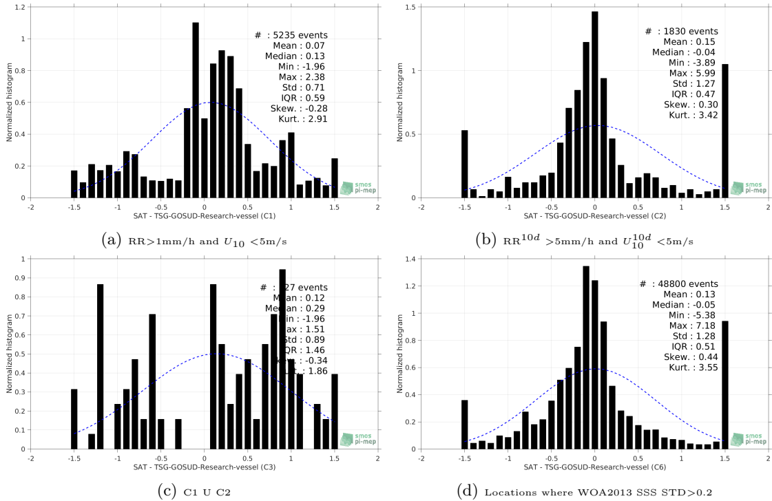
Figure 13: Normalized histogram of \Delta SSS (SMAP-L3-RSS-V3-MONTHLY-70KM - TSG-GOSUD-Research-vessel) for 6 different subdatasets corresponding to: RR>1mm/h and U_{10} < 5\text{m/s} (a), RR^{10d} > 5\text{mm/h} and U_{10}^{10d} < 5\text{m/s} (b), C1 U C2 (c), Locations where WOA2013 SSS STD>0.2 (d).
