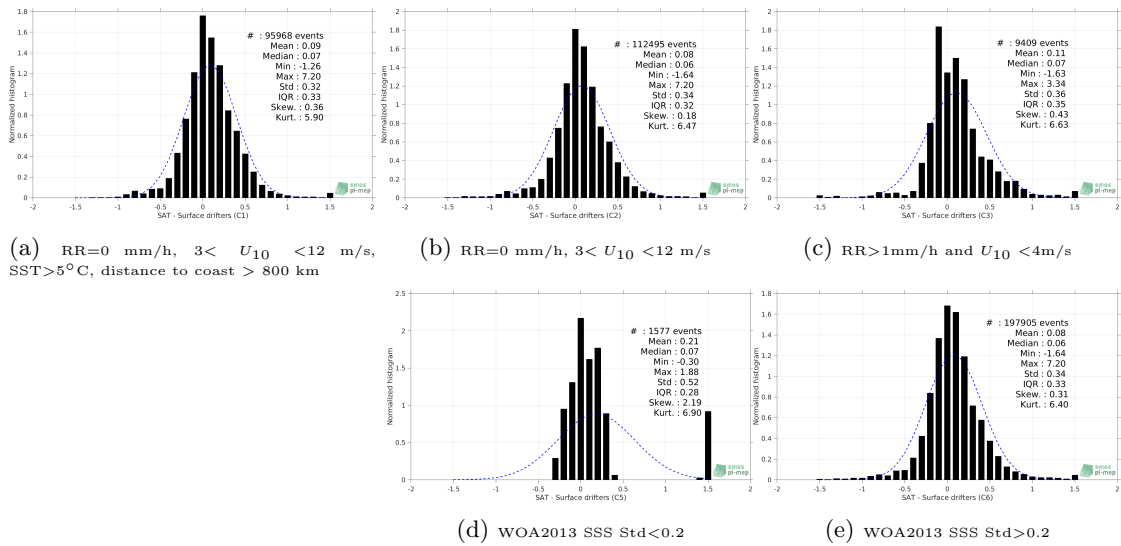
Figure 12: Normalized histogram of \Delta SSS (SMAP-L3-RSS-V3-MONTHLY-70KM - Surface drifters) for 5 different subdatasets corresponding to: RR=0 mm/h, 3 < U_{10} < 12 m/s, SST > 5^\circ C , distance to coast > 800 km (a), RR=0 mm/h, 3 < U_{10} < 12 m/s (b), RR>1mm/h and U_{10} < 4 m/s (c), WOA2013 SSS Std<0.2 (d), WOA2013 SSS Std>0.2 (e).
