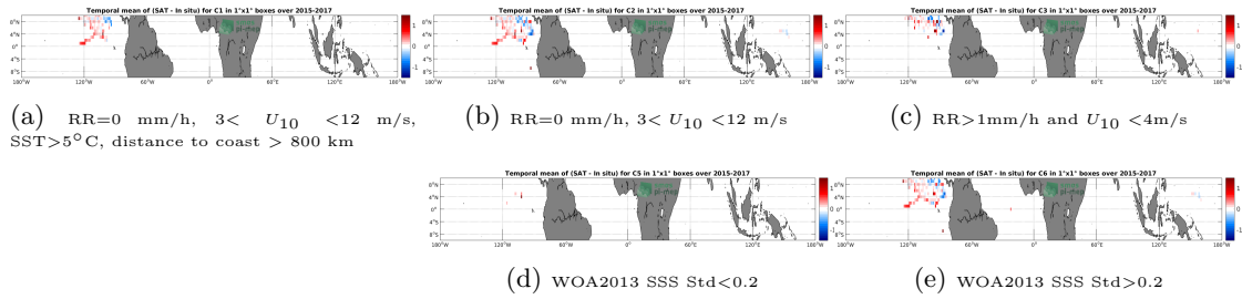
Figure 11: Temporal mean gridded over spatial boxes of size 1^\circ \times 1^\circ of \Delta SSS (SMAP-L3-RSS-V3-MONTHLY-70KM - Surface drifters) for 5 different subdatasets corresponding to:RR=0 mm/h, 3 < U_{10} < 12 m/s, SST > 5^\circ C , distance to coast > 800 km (a), RR=0 mm/h, 3 < U_{10} < 12 m/s (b), RR>1mm/h and U_{10} < 4 m/s (c), WOA2013 SSS Std<0.2 (d), WOA2013 SSS Std>0.2 (e).
