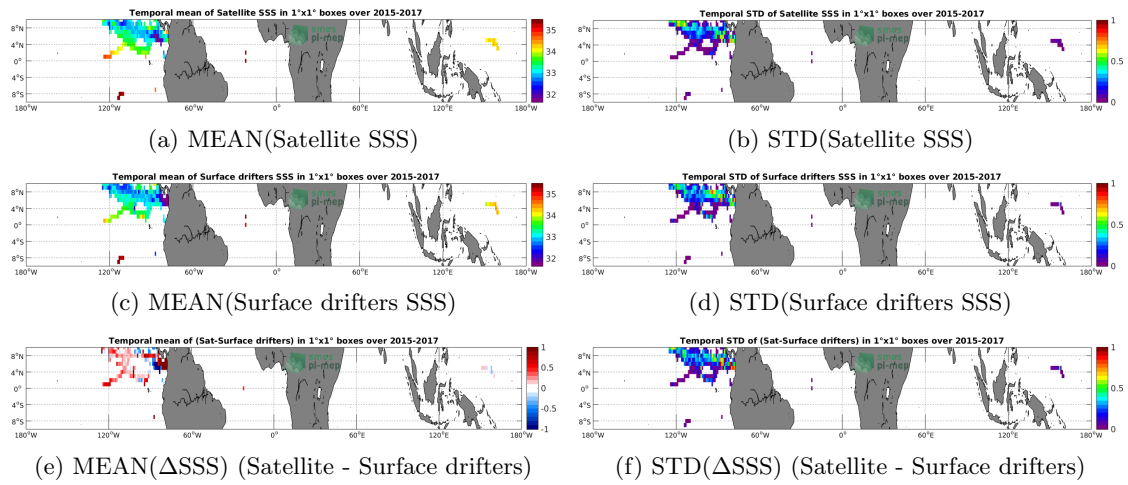
Figure 5: Temporal mean (left) and STD (right) of SSS from SMAP-L3-RSS-V3-MONTHLY-70KM (top), Surface drifters (middle), and of \Delta SSS (Satellite - Surface drifters). Only match-up pairs are used to generate these maps.
