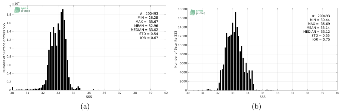
Figure 2: Histograms of SSS from Surface drifters (a) and SMAP-L3-RSS-V3-MONTHLY-70KM (b) considering all match-up pairs per bins of 0.1 over the Equatorial Ocean 10N-10S Pi-MEP region and for the full satellite product period.
