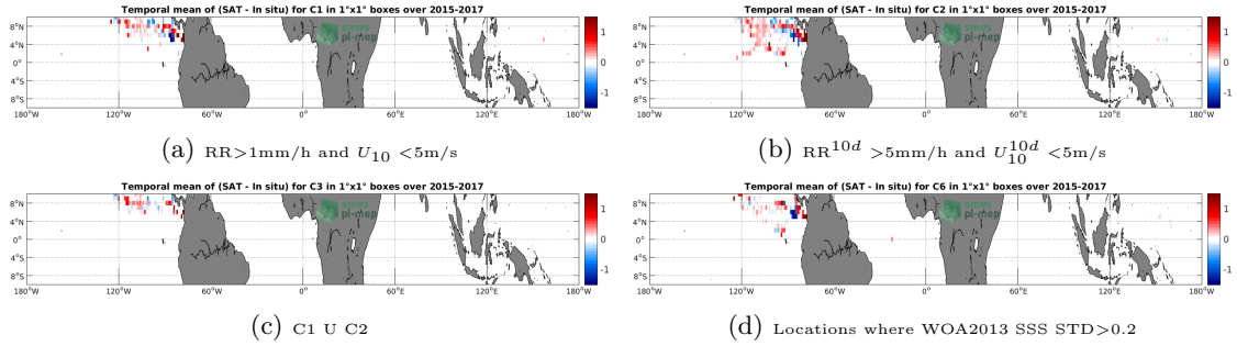
Figure 11: Temporal mean gridded over spatial boxes of size 1^\circ \times 1^\circ of \Delta SSS (SMAP-L3-RSS-V3-MONTHLY-70KM - Surface drifters) for 4 different subdatasets corresponding to: RR>1mm/h and U_{10} < 5m/s (a), RR^{10d} > 5mm/h and U_{10}^{10d} < 5m/s (b), C1 U C2 (c), Locations where WOA2013 SSS STD>0.2 (d).
