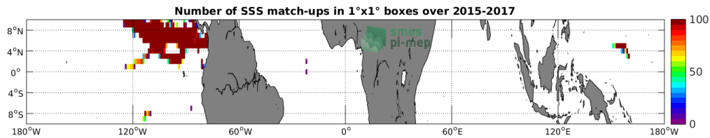
Figure 3: Number of SSS match-ups between Surface drifters SSS and the SMAP-L3-RSS-V3-MONTHLY-70KM SSS product for the Equatorial Ocean 10N-10S Pi-MEP region over 1°x1° boxes and for the full satellite product period.
