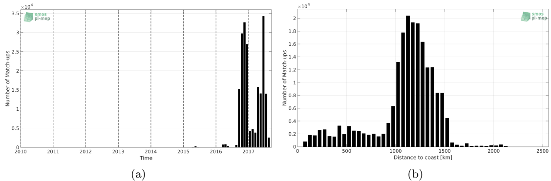
Figure 1: Number of match-ups between Surface drifters and SMAP-L3-RSS-V3-MONTHLY-70KM SSS as a function of time (a) and as function of the distance to coast (b) over the Equatorial Ocean 10N-10S Pi-MEP region and for the full satellite product period.
