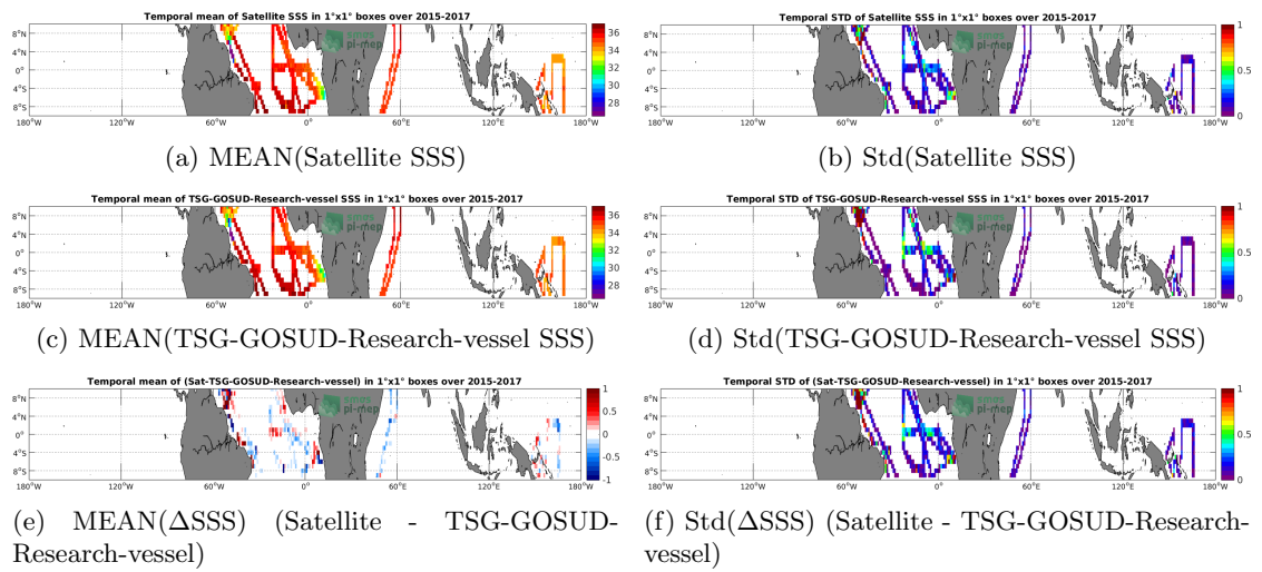
Figure 6: Temporal mean (left) and Std (right) of SSS from SMAP-L3-RSS-V3-MONTHLY-0.25DEG-40KM (top), TSG-GOSUD-Research-vessel (middle), and of \Delta SSS (Satellite - TSG-GOSUD-Research-vessel). Only match-up pairs are used to generate these maps.
