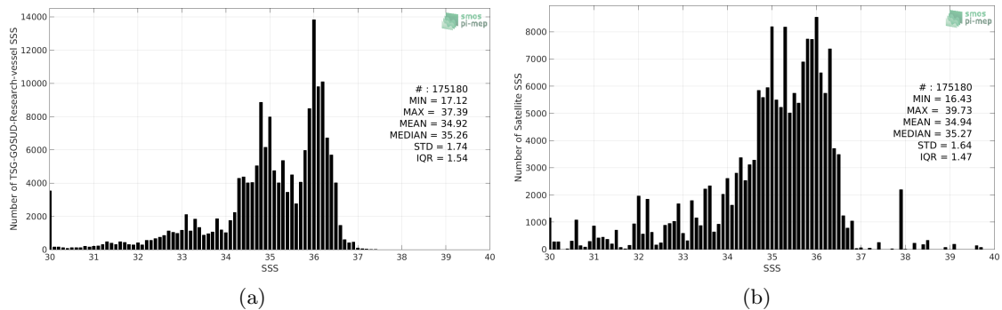
Figure 2: Histograms of SSS from TSG-GOSUD-Research-vessel (a) and SMAP-L3-RSS-V3-MONTHLY-0.25DEG-40KM (b) considering all match-up pairs per bins of 0.1 over the Equatorial Ocean 10N-10S Pi-MEP region and for the full satellite product period.
