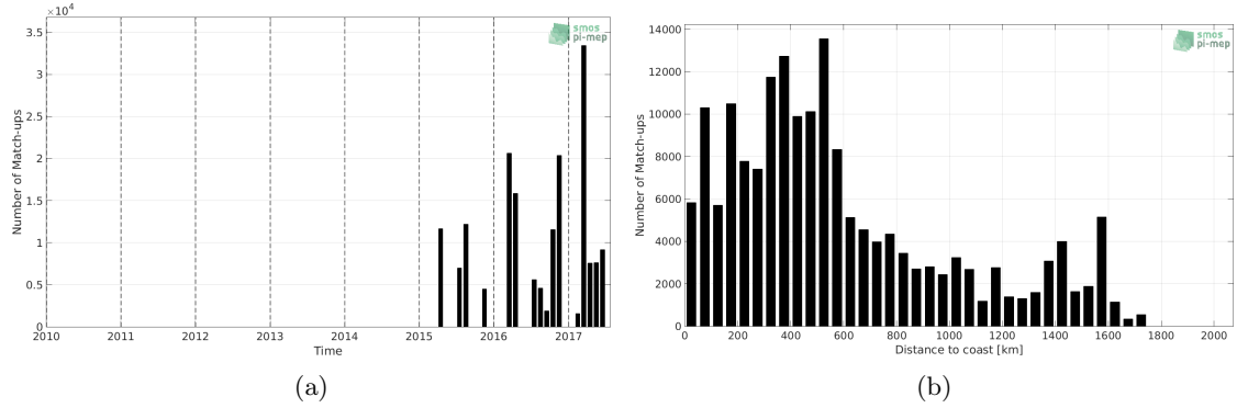
Figure 1: Number of match-ups between TSG-GOSUD-Research-vessel and SMAP-L3-RSS-V3-MONTHLY-0.25DEG-40KM SSS as a function of time (a) and as function of the distance to coast (b) over the Equatorial Ocean 10N-10S Pi-MEP region and for the full satellite product period.
