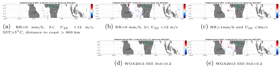
Figure 12: Temporal mean gridded over spatial boxes of size 1^\circ \times 1^\circ of \Delta SSS (SMAP-L3-RSS-V3-MONTHLY-0.25DEG-40KM - TSG-GOSUD-Research-vessel) for 5 different subdatasets corresponding to: RR=0 mm/h, 3 < U_{10} < 12 m/s, SST > 5^\circ C , distance to coast > 800 km (a), RR=0 mm/h, 3 < U_{10} < 12 m/s (b), RR > 1 mm/h and U_{10} < 4 m/s (c), WOA2013 SSS Std < 0.2 (d), WOA2013 SSS Std > 0.2 (e).
