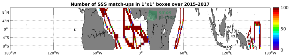
Figure 4: Number of SSS match-ups between TSG-GOSUD-Research-vessel SSS and the SMAP-L3-RSS-V3-MONTHLY-0.25DEG-40KM SSS product for the Equatorial Ocean 10N-10S Pi-MEP region over 1^\circ \times 1^\circ boxes and for the full satellite product period.
