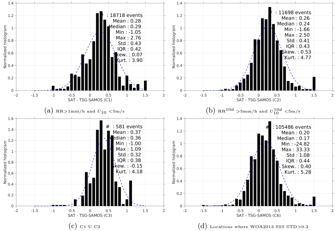
Figure 13: Normalized histogram of \Delta\text{SSS} (SMAP-L3-RSS-V2-8DAY-RUNNING-40KM - TSG-SAMOS) for 6 different subdatasets corresponding to: \text{RR} > 1\text{mm/h} and U_{10} < 5\text{m/s} (a), \text{RR}^{10d} > 5\text{mm/h} and U_{10}^{10d} < 5\text{m/s} (b), C1 U C2 (c), Locations where WOA2013 SSS STD > 0.2 (d).
