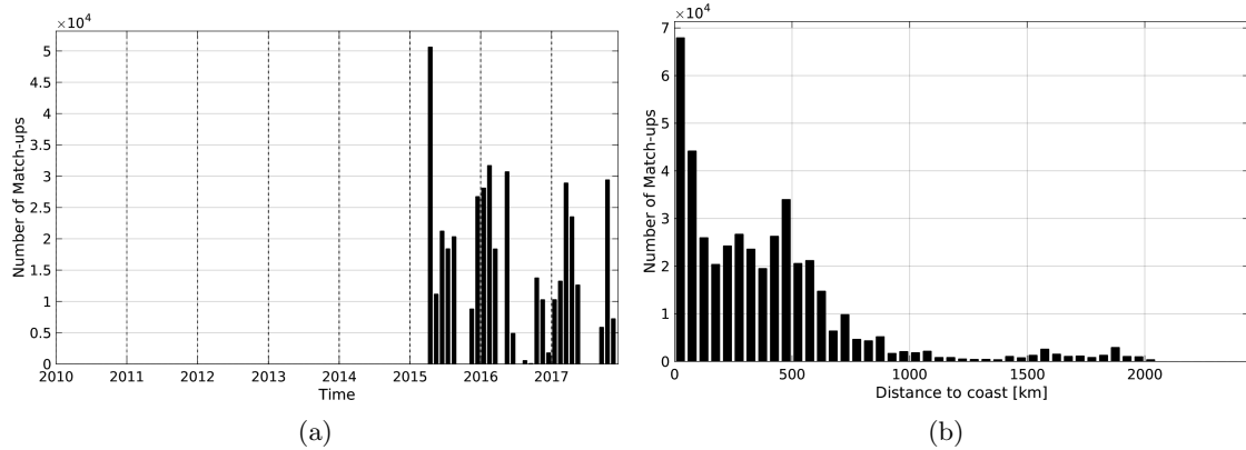
Figure 1: Number of match-ups between TSG-SAMOS and SMAP-L3-RSS-V2-8DAY-RUNNING-40KM SSS as a function of time (a) and as function of the distance to coast (b) over the Equatorial Ocean 10N-10S Pi-MEP region and for the full satellite product period.
