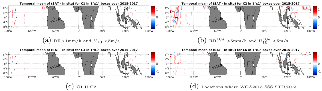
Figure 12: Temporal mean gridded over spatial boxes of size 1^\circ \times 1^\circ of \Delta SSS (SMAP-L3-RSS-V2-8DAY-RUNNING-40KM - TSG-SAMOS) for 4 different subdatasets corresponding to: RR > 1\text{mm/h} and U_{10} < 5\text{m/s} (a), RR^{10d} > 5\text{mm/h} and U_{10}^{10d} < 5\text{m/s} (b), C1 U C2 (c), Locations where WOA2013 SSS STD > 0.2 (d).
