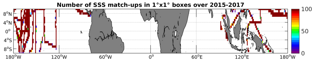
Figure 4: Number of SSS match-ups between TSG-SAMOS SSS and the SMAP-L3-RSS-V2-8DAY-RUNNING-40KM SSS product for the Equatorial Ocean 10N-10S Pi-MEP region over 1^\circ \times 1^\circ boxes and for the full satellite product period.
