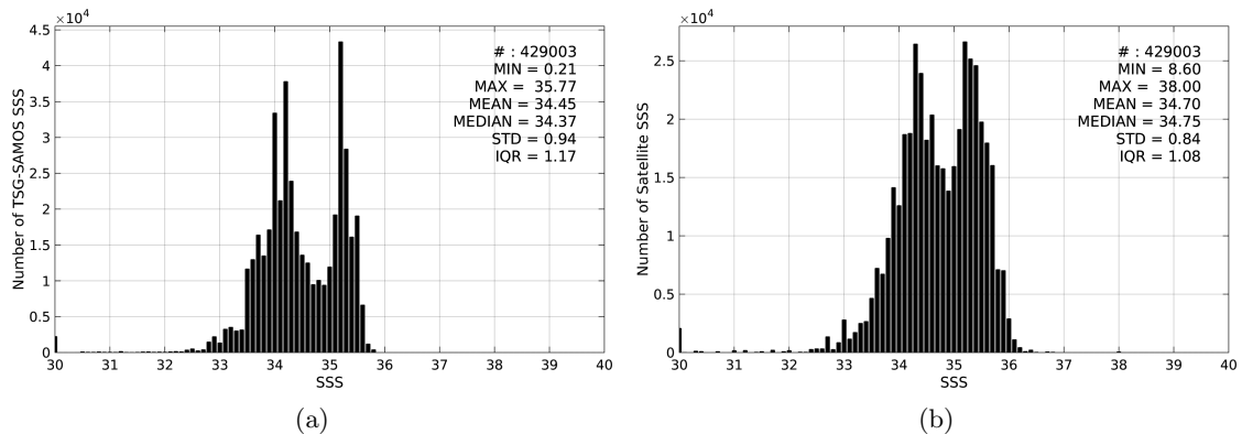
Figure 2: Histograms of SSS from TSG-SAMOS (a) and SMAP-L3-RSS-V2-8DAY-RUNNING-40KM (b) considering all match-up pairs per bins of 0.1 over the Equatorial Ocean 10N-10S Pi-MEP region and for the full satellite product period.
