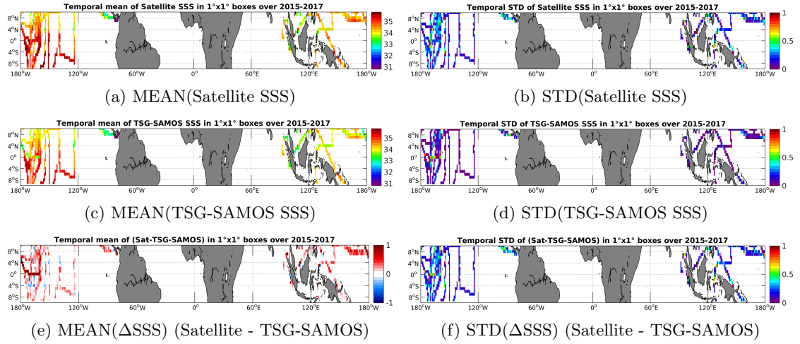
Figure 6: Temporal mean (left) and STD (right) of SSS from SMAP-L3-RSS-V2-8DAY-RUNNING-40KM (top), TSG-SAMOS (middle), and of \Delta SSS (Satellite - TSG-SAMOS). Only match-up pairs are used to generate these maps.
