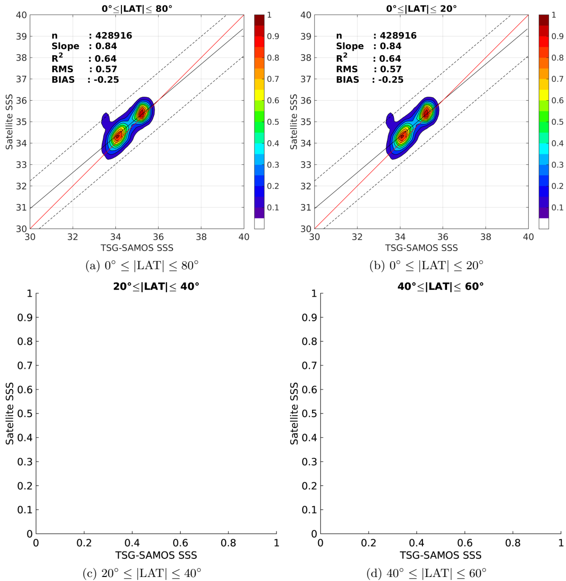
Figure 9: Contour maps of the concentration of SMAP-L3-RSS-V2-8DAY-RUNNING-40KM SSS (y-axis) versus TSG-SAMOS SSS (x-axis) at match-up pairs for different latitude bands. For each plot, the red line shows x=y . The black thin and dashed lines indicate a linear fit through the data cloud and the \pm 95\% confidence levels, respectively. The number match-up pairs n , the slope and R^2 coefficient of the linear fit, the root mean square (RMS) and the mean bias between satellite and in situ data are indicated for each latitude band in each plots.
