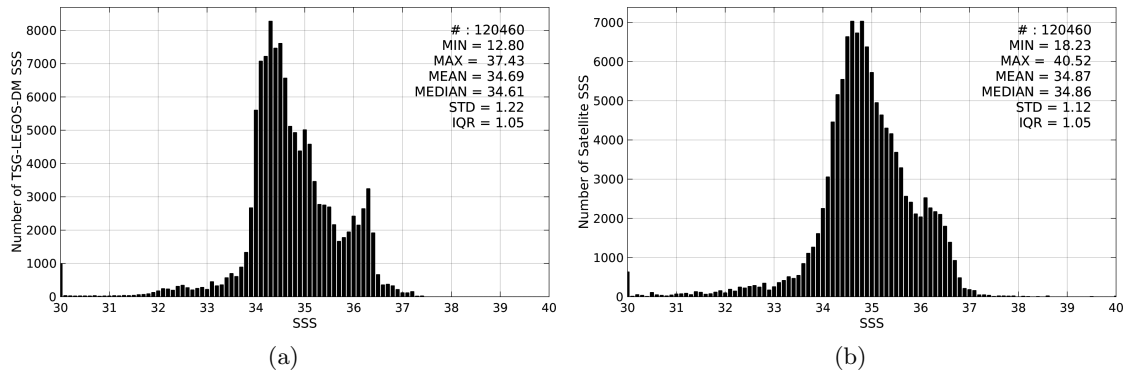
Figure 2: Histograms of SSS from TSG-LEGOS-DM (a) and SMAP-L3-RSS-V2-8DAY-RUNNING-40KM (b) considering all match-up pairs per bins of 0.1 over the Equatorial Ocean 10N-10S Pi-MEP region and for the full satellite product period.
