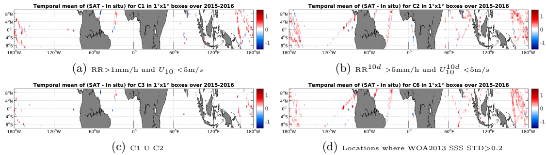
Figure 12: Temporal mean gridded over spatial boxes of size 1^\circ \times 1^\circ of \Delta SSS (SMAP-L3-RSS-V2-8DAY-RUNNING-40KM - TSG-LEGOS-DM) for 4 different subdatasets corresponding to: RR > 1\text{mm/h} and U_{10} < 5\text{m/s} (a), RR^{10d} > 5\text{mm/h} and U_{10}^{10d} < 5\text{m/s} (b), C1 U C2 (c), Locations where WOA2013 SSS STD > 0.2 (d).
