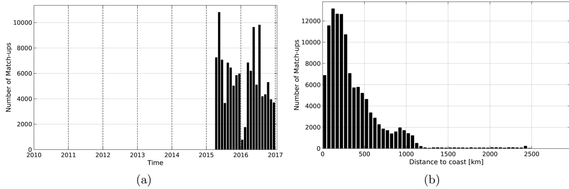
Figure 1: Number of match-ups between TSG-LEGOS-DM and SMAP-L3-RSS-V2-8DAY-RUNNING-40KM SSS as a function of time (a) and as function of the distance to coast (b) over the Equatorial Ocean 10N-10S Pi-MEP region and for the full satellite product period.
