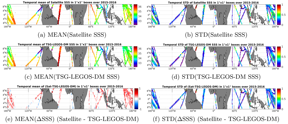
Figure 6: Temporal mean (left) and STD (right) of SSS from SMAP-L3-RSS-V2-8DAY-RUNNING-40KM (top), TSG-LEGOS-DM (middle), and of \Delta SSS (Satellite - TSG-LEGOS-DM). Only match-up pairs are used to generate these maps.
