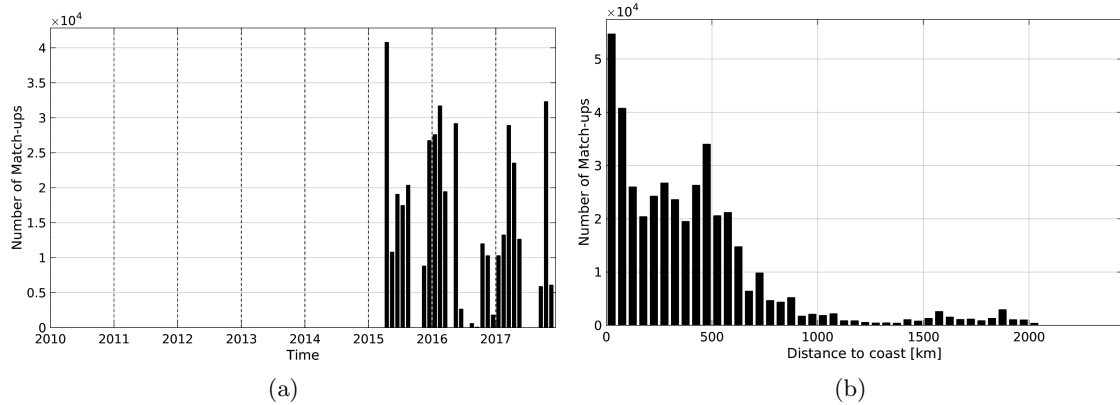
Figure 1: Number of match-ups between TSG-SAMOS and SMAP-L3-RSS-V2-8DAY-RUNNING-70KM SSS as a function of time (a) and as function of the distance to coast (b) over the Equatorial Ocean 10N-10S Pi-MEP region and for the full satellite product period.
