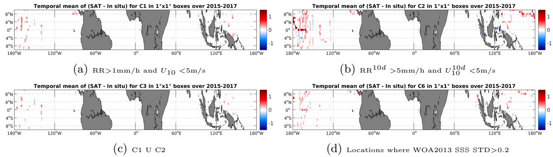
Figure 12: Temporal mean gridded over spatial boxes of size 1^\circ \times 1^\circ of \Delta SSS (SMAP-L3-RSS-V2-8DAY-RUNNING-70KM - TSG-SAMOS) for 4 different subdatasets corresponding to: RR > 1\text{mm/h} and U_{10} < 5\text{m/s} (a), RR^{10d} > 5\text{mm/h} and U_{10}^{10d} < 5\text{m/s} (b), C1 U C2 (c), Locations where WOA2013 SSS STD > 0.2 (d).
