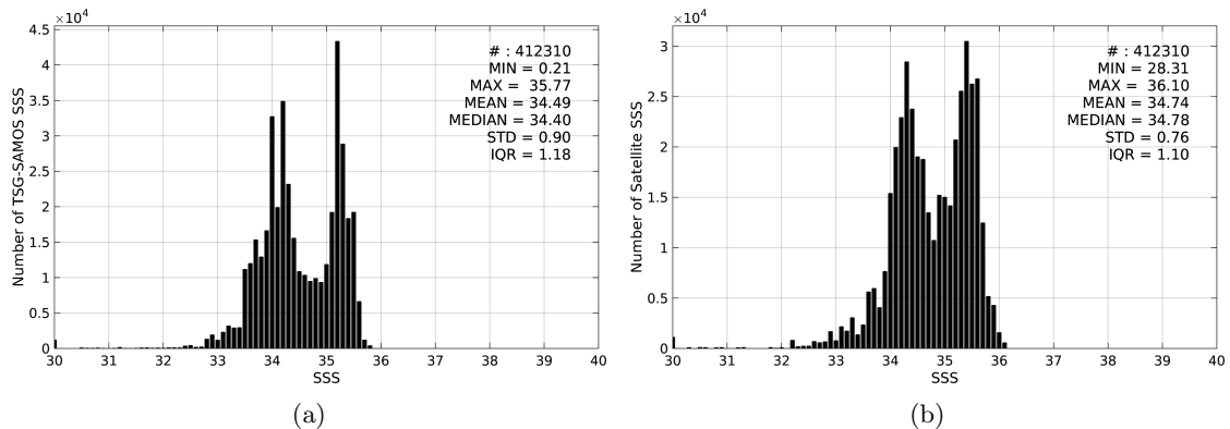
Figure 2: Histograms of SSS from TSG-SAMOS (a) and SMAP-L3-RSS-V2-8DAY-RUNNING-70KM (b) considering all match-up pairs per bins of 0.1 over the Equatorial Ocean 10N-10S Pi-MEP region and for the full satellite product period.
