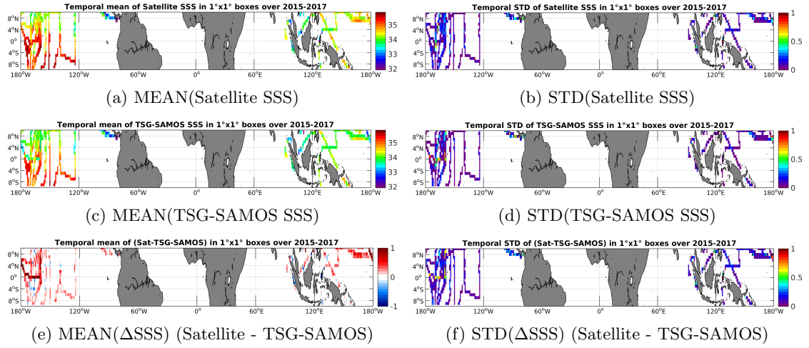
Figure 6: Temporal mean (left) and STD (right) of SSS from SMAP-L3-RSS-V2-8DAY-RUNNING-70KM (top), TSG-SAMOS (middle), and of \Delta SSS (Satellite - TSG-SAMOS). Only match-up pairs are used to generate these maps.
