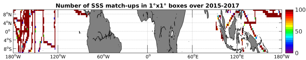
Figure 4: Number of SSS match-ups between TSG-SAMOS SSS and the SMAP-L3-RSS-V2-8DAY-RUNNING-70KM SSS product for the Equatorial Ocean 10N-10S Pi-MEP region over 1^\circ \times 1^\circ boxes and for the full satellite product period.
