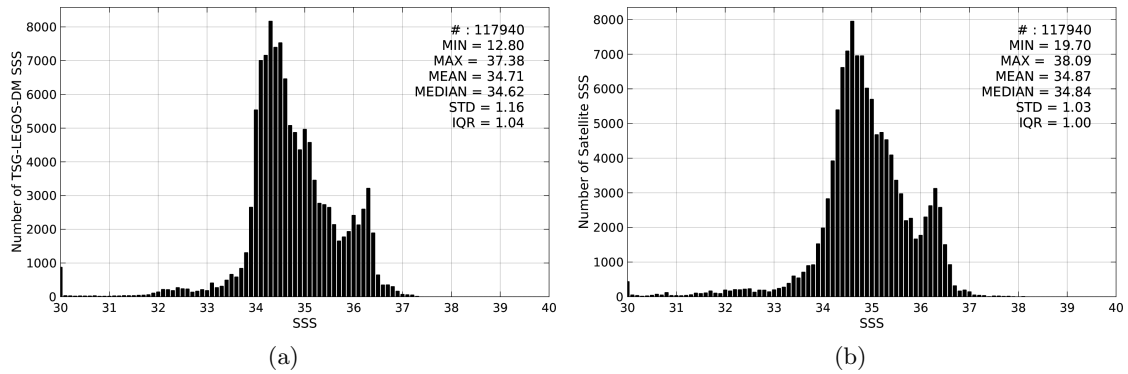
Figure 2: Histograms of SSS from TSG-LEGOS-DM (a) and SMAP-L3-RSS-V2-8DAY-RUNNING-70KM (b) considering all match-up pairs per bins of 0.1 over the Equatorial Ocean 10N-10S Pi-MEP region and for the full satellite product period.
