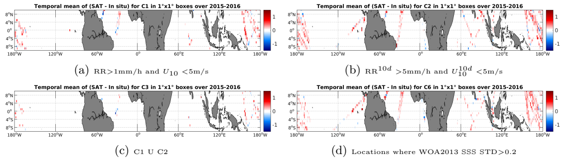
Figure 12: Temporal mean gridded over spatial boxes of size 1^\circ \times 1^\circ of \Delta SSS (SMAP-L3-RSS-V2-8DAY-RUNNING-70KM - TSG-LEGOS-DM) for 4 different subdatasets corresponding to: RR > 1\text{mm/h} and U_{10} < 5\text{m/s} (a), RR^{10d} > 5\text{mm/h} and U_{10}^{10d} < 5\text{m/s} (b), C1 U C2 (c), Locations where WOA2013 SSS STD > 0.2 (d).
