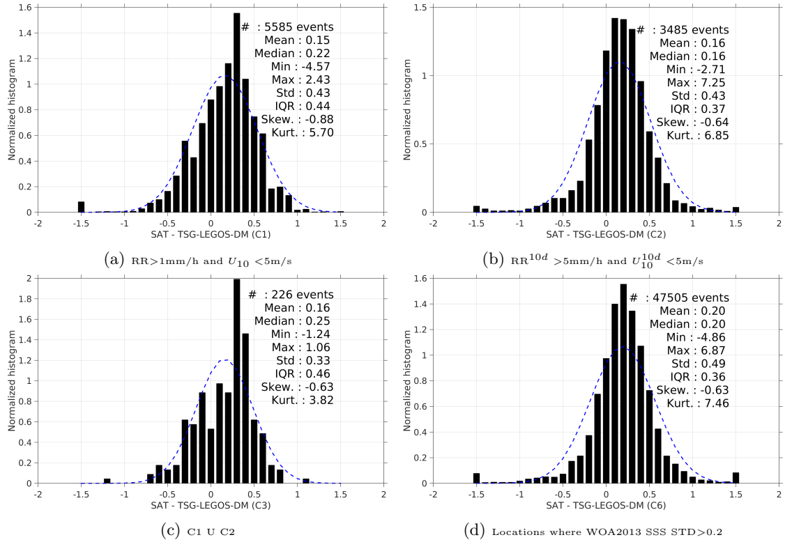
Figure 13: Normalized histogram of \Delta\text{SSS} (SMAP-L3-RSS-V2-8DAY-RUNNING-70KM - TSG-LEGOS-DM) for 6 different subdatasets corresponding to: \text{RR} > 1\text{mm/h} and U_{10} < 5\text{m/s} (a), \text{RR}^{10d} > 5\text{mm/h} and U_{10}^{10d} < 5\text{m/s} (b), C1 U C2 (c), Locations where WOA2013 SSS STD > 0.2 (d).
