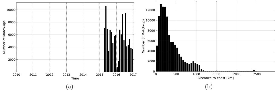
Figure 1: Number of match-ups between TSG-LEGOS-DM and SMAP-L3-RSS-V2-8DAY-RUNNING-70KM SSS as a function of time (a) and as function of the distance to coast (b) over the Equatorial Ocean 10N-10S Pi-MEP region and for the full satellite product period.
