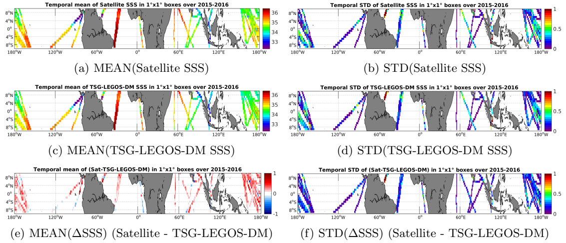
Figure 6: Temporal mean (left) and STD (right) of SSS from SMAP-L3-RSS-V2-8DAY-RUNNING-70KM (top), TSG-LEGOS-DM (middle), and of \Delta SSS (Satellite - TSG-LEGOS-DM). Only match-up pairs are used to generate these maps.
