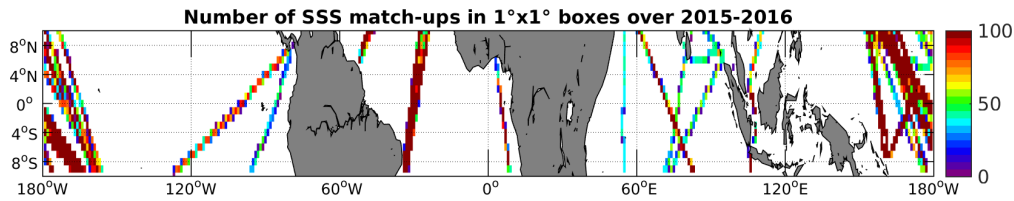
Figure 4: Number of SSS match-ups between TSG-LEGOS-DM SSS and the SMAP-L3-RSS-V2-8DAY-RUNNING-70KM SSS product for the Equatorial Ocean 10N-10S Pi-MEP region over 1^\circ \times 1^\circ boxes and for the full satellite product period.
