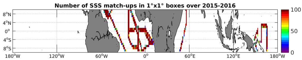
Figure 4: Number of SSS match-ups between TSG-GOSUD-Research-vessel SSS and the SMAP-L3-RSS-V2-8DAY-RUNNING-70KM SSS product for the Equatorial Ocean 10N-10S Pi-MEP region over 1°x1° boxes and for the full satellite product period.
