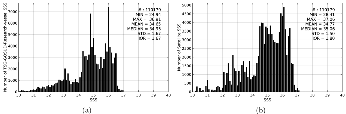
Figure 2: Histograms of SSS from TSG-GOSUD-Research-vessel (a) and SMAP-L3-RSS-V2-8DAY-RUNNING-70KM (b) considering all match-up pairs per bins of 0.1 over the Equatorial Ocean 10N-10S Pi-MEP region and for the full satellite product period.
