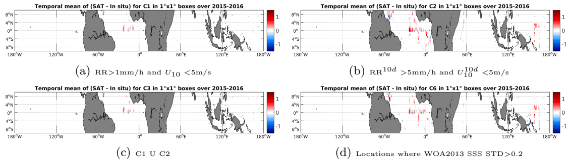
Figure 12: Temporal mean gridded over spatial boxes of size 1^\circ \times 1^\circ of \Delta SSS (SMAP-L3-RSS-V2-8DAY-RUNNING-70KM - TSG-GOSUD-Research-vessel) for 4 different subdatasets corresponding to: RR > 1\text{mm/h} and U_{10} < 5\text{m/s} (a), RR^{10d} > 5\text{mm/h} and U_{10}^{10d} < 5\text{m/s} (b), C1 U C2 (c), Locations where WOA2013 SSS STD > 0.2 (d).
