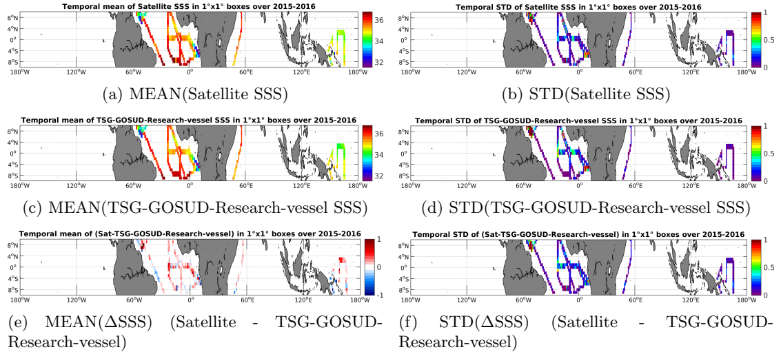
Figure 6: Temporal mean (left) and STD (right) of SSS from SMAP-L3-RSS-V2-8DAY-RUNNING-70KM (top), TSG-GOSUD-Research-vessel (middle), and of \Delta SSS (Satellite - TSG-GOSUD-Research-vessel). Only match-up pairs are used to generate these maps.
