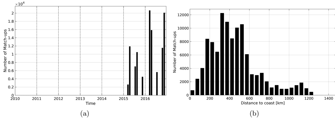
Figure 1: Number of match-ups between TSG-GOSUD-Research-vessel and SMAP-L3-RSS-V2-8DAY-RUNNING-70KM SSS as a function of time (a) and as function of the distance to coast (b) over the Equatorial Ocean 10N-10S Pi-MEP region and for the full satellite product period.
