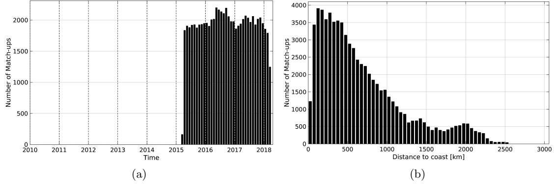
Figure 1: Number of match-ups between Argo and SMAP-L3-RSS-V2-8DAY-RUNNING-70KM SSS as a function of time (a) and as function of the distance to coast (b) over the Equatorial Ocean 10N-10S Pi-MEP region and for the full satellite product period.
