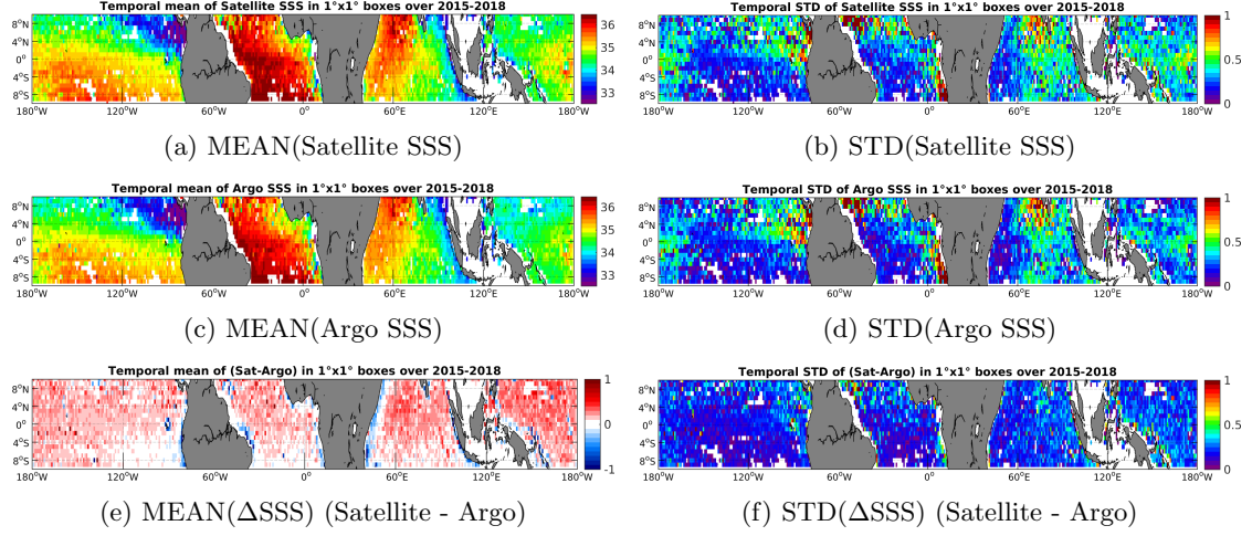
Figure 6: Temporal mean (left) and STD (right) of SSS from SMAP-L3-RSS-V2-8DAY-RUNNING-70KM (top), Argo (middle), and of \Delta SSS (Satellite - Argo). Only match-up pairs are used to generate these maps.
