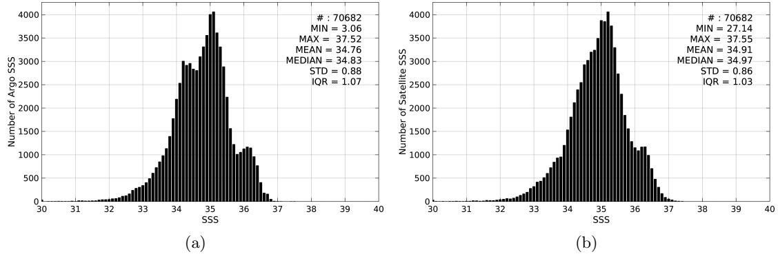
Figure 2: Histograms of SSS from Argo (a) and SMAP-L3-RSS-V2-8DAY-RUNNING-70KM (b) considering all match-up pairs per bins of 0.1 over the Equatorial Ocean 10N-10S Pi-MEP region and for the full satellite product period.
