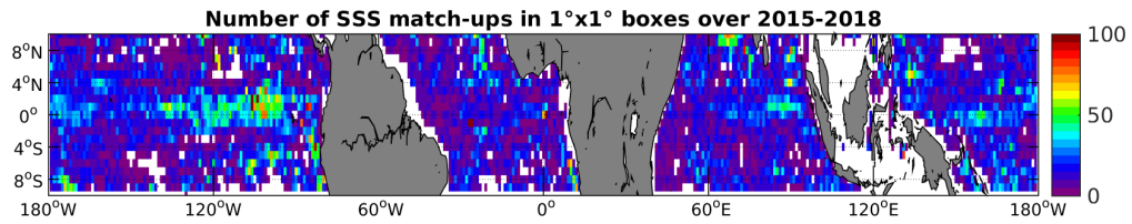
Figure 4: Number of SSS match-ups between Argo SSS and the SMAP-L3-RSS-V2-8DAY-RUNNING-70KM SSS product for the Equatorial Ocean 10N-10S Pi-MEP region over 1^\circ \times 1^\circ boxes and for the full satellite product period.
