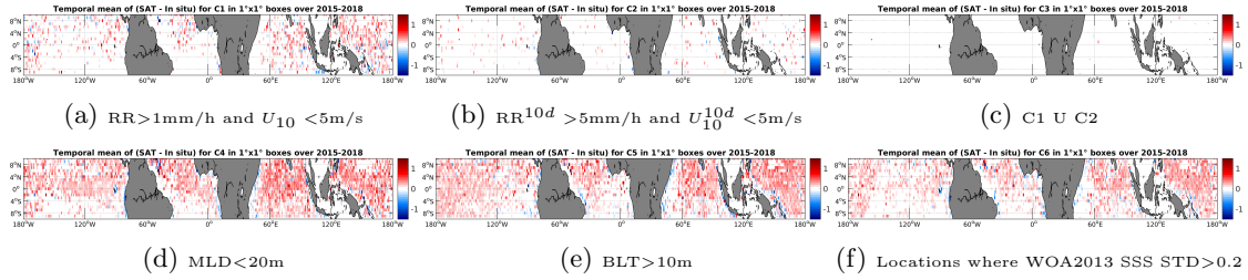
Figure 12: Temporal mean gridded over spatial boxes of size 1^\circ \times 1^\circ of \Delta SSS (SMAP-L3-RSS-V2-8DAY-RUNNING-70KM - Argo) for 6 different subdatasets corresponding to: RR > 1\text{mm/h} and U_{10} < 5\text{m/s} (a), RR^{10d} > 5\text{mm/h} and U_{10}^{10d} < 5\text{m/s} (b), C1 U C2 (c), MLD < 20\text{m} (d), BLT > 10\text{m} (e), Locations where WOA2013 SSS STD > 0.2 (f).
