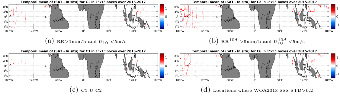
Figure 12: Temporal mean gridded over spatial boxes of size 1^\circ \times 1^\circ of \Delta SSS (SMAP-L3-RSS-V2-MONTHLY-0.25DEG-40KM - TSG-SAMOS) for 4 different subdatasets corresponding to: RR > 1 mm/h and U_{10} < 5 m/s (a), RR^{10d} > 5 mm/h and U_{10}^{10d} < 5 m/s (b), C1 U C2 (c), Locations where WOA2013 SSS STD > 0.2 (d).
