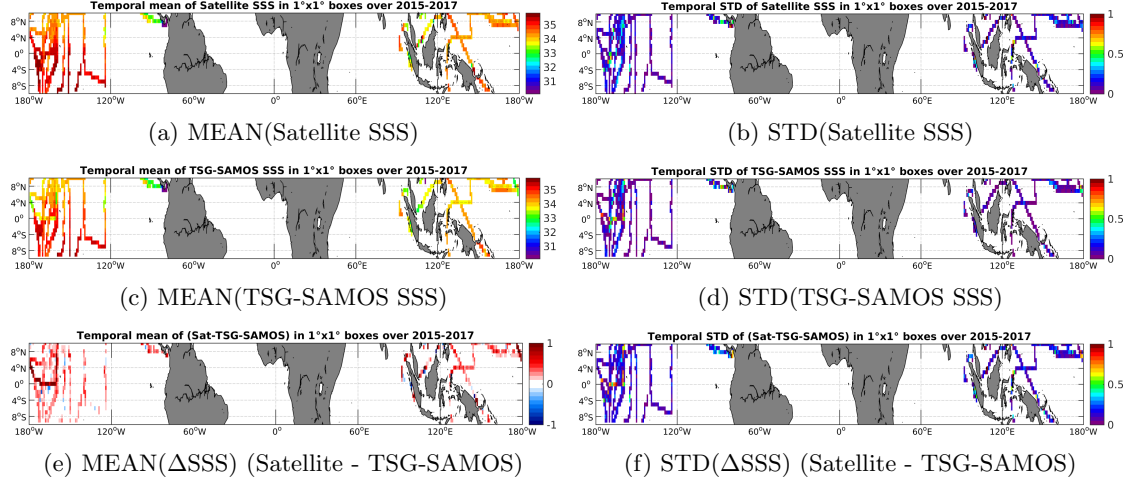
Figure 6: Temporal mean (left) and STD (right) of SSS from SMAP-L3-RSS-V2-MONTHLY-0.25DEG-40KM (top), TSG-SAMOS (middle), and of \Delta SSS (Satellite - TSG-SAMOS). Only match-up pairs are used to generate these maps.
