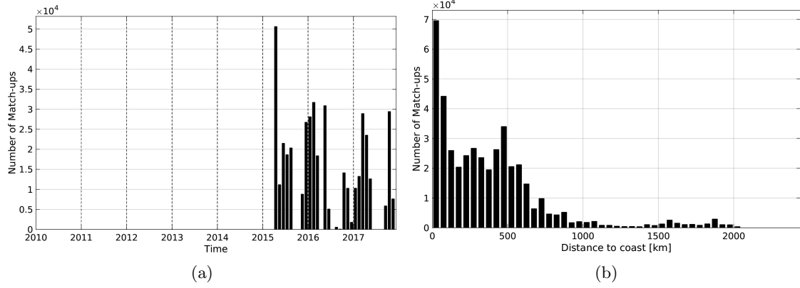
Figure 1: Number of match-ups between TSG-SAMOS and SMAP-L3-RSS-V2-MONTHLY-0.25DEG-40KM SSS as a function of time (a) and as function of the distance to coast (b) over the Equatorial Ocean 10N-10S Pi-MEP region and for the full satellite product period.
