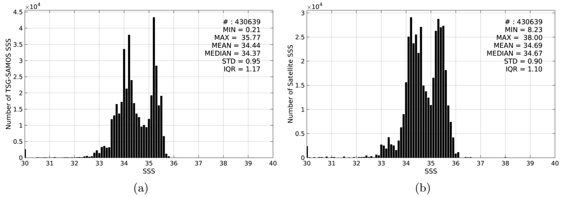
Figure 2: Histograms of SSS from TSG-SAMOS (a) and SMAP-L3-RSS-V2-MONTHLY-0.25DEG-40KM (b) considering all match-up pairs per bins of 0.1 over the Equatorial Ocean 10N-10S Pi-MEP region and for the full satellite product period.
