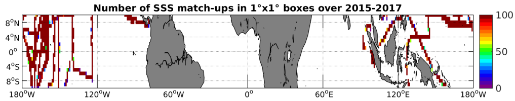
Figure 4: Number of SSS match-ups between TSG-SAMOS SSS and the SMAP-L3-RSS-V2-MONTHLY-0.25DEG-40KM SSS product for the Equatorial Ocean 10N-10S Pi-MEP region over 1^\circ \times 1^\circ boxes and for the full satellite product period.
