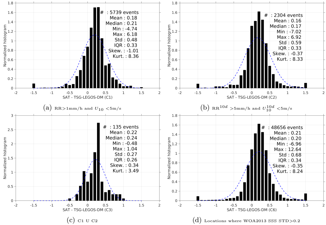
Figure 13: Normalized histogram of \Delta SSS (SMAP-L3-RSS-V2-MONTHLY-0.25DEG-40KM - TSG-LEGOS-DM) for 6 different subdatasets corresponding to: RR > 1\text{mm/h} and U_{10} < 5\text{m/s} (a), RR^{10d} > 5\text{mm/h} and U_{10}^{10d} < 5\text{m/s} (b), C1 U C2 (c), Locations where WOA2013 SSS STD > 0.2 (d).
