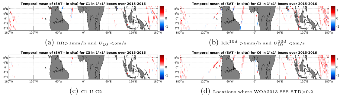
Figure 12: Temporal mean gridded over spatial boxes of size 1^\circ \times 1^\circ of \Delta SSS (SMAP-L3-RSS-V2-MONTHLY-0.25DEG-40KM - TSG-LEGOS-DM) for 4 different subdatasets corresponding to: RR > 1\text{mm/h} and U_{10} < 5\text{m/s} (a), RR^{10d} > 5\text{mm/h} and U_{10}^{10d} < 5\text{m/s} (b), C1 U C2 (c), Locations where WOA2013 SSS STD > 0.2 (d).
