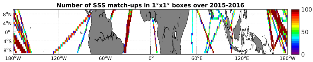
Figure 4: Number of SSS match-ups between TSG-LEGOS-DM SSS and the SMAP-L3-RSS-V2-MONTHLY-0.25DEG-40KM SSS product for the Equatorial Ocean 10N-10S Pi-MEP region over 1^\circ \times 1^\circ boxes and for the full satellite product period.
