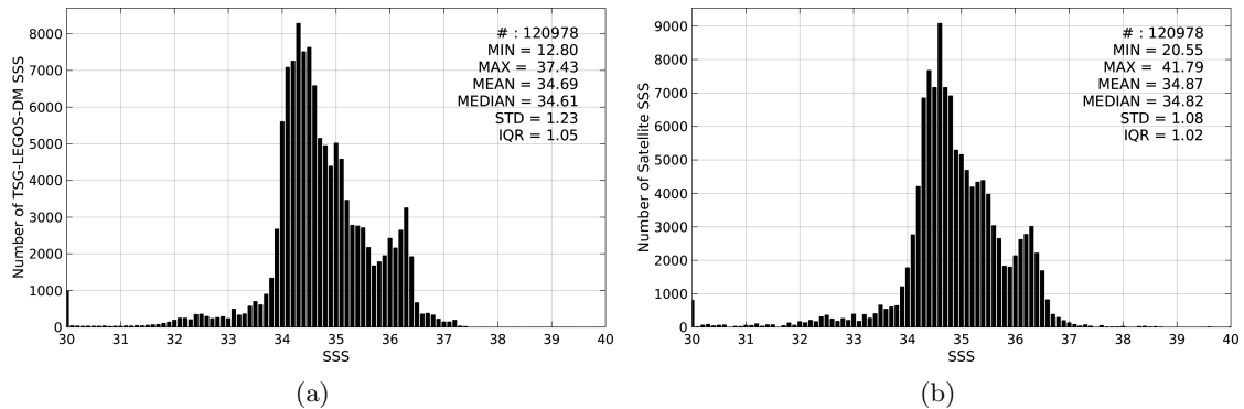
Figure 2: Histograms of SSS from TSG-LEGOS-DM (a) and SMAP-L3-RSS-V2-MONTHLY-0.25DEG-40KM (b) considering all match-up pairs per bins of 0.1 over the Equatorial Ocean 10N-10S Pi-MEP region and for the full satellite product period.
