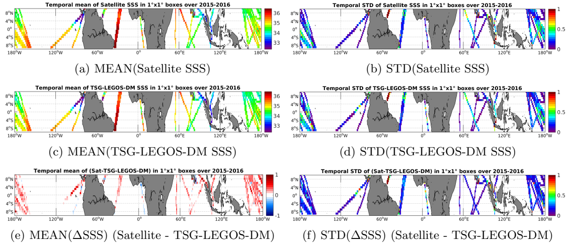
Figure 6: Temporal mean (left) and STD (right) of SSS from SMAP-L3-RSS-V2-MONTHLY-0.25DEG-40KM (top), TSG-LEGOS-DM (middle), and of \Delta SSS (Satellite - TSG-LEGOS-DM). Only match-up pairs are used to generate these maps.
