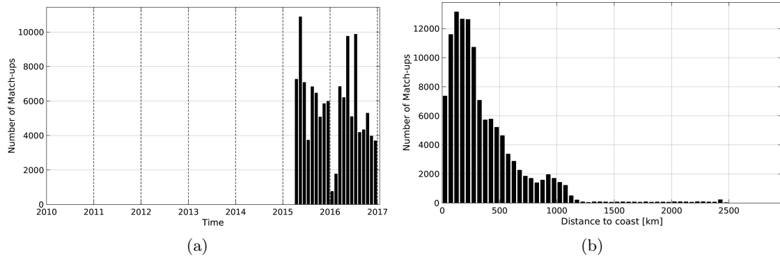
Figure 1: Number of match-ups between TSG-LEGOS-DM and SMAP-L3-RSS-V2-MONTHLY-0.25DEG-40KM SSS as a function of time (a) and as function of the distance to coast (b) over the Equatorial Ocean 10N-10S Pi-MEP region and for the full satellite product period.
