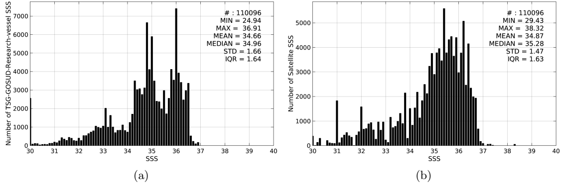
Figure 2: Histograms of SSS from TSG-GOSUD-Research-vessel (a) and SMAP-L3-RSS-V2-MONTHLY-0.25DEG-40KM (b) considering all match-up pairs per bins of 0.1 over the Equatorial Ocean 10N-10S Pi-MEP region and for the full satellite product period.
