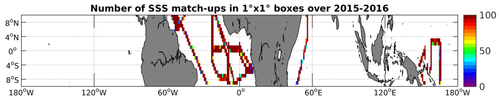
Figure 4: Number of SSS match-ups between TSG-GOSUD-Research-vessel SSS and the SMAP-L3-RSS-V2-MONTHLY-0.25DEG-40KM SSS product for the Equatorial Ocean 10N-10S Pi-MEP region over 1°x1° boxes and for the full satellite product period.
