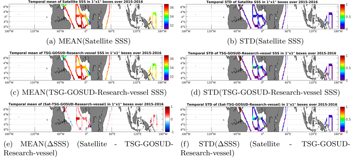
Figure 6: Temporal mean (left) and STD (right) of SSS from SMAP-L3-RSS-V2-MONTHLY-0.25DEG-40KM (top), TSG-GOSUD-Research-vessel (middle), and of \Delta SSS (Satellite - TSG-GOSUD-Research-vessel). Only match-up pairs are used to generate these maps.
