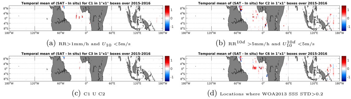
Figure 12: Temporal mean gridded over spatial boxes of size 1^\circ \times 1^\circ of \Delta SSS (SMAP-L3-RSS-V2-MONTHLY-0.25DEG-40KM - TSG-GOSUD-Research-vessel) for 4 different subdatasets corresponding to: RR > 1mm/h and U_{10} < 5 m/s (a), RR^{10d} > 5 mm/h and U_{10}^{10d} < 5 m/s (b), C1 U C2 (c), Locations where WOA2013 SSS STD > 0.2 (d).
