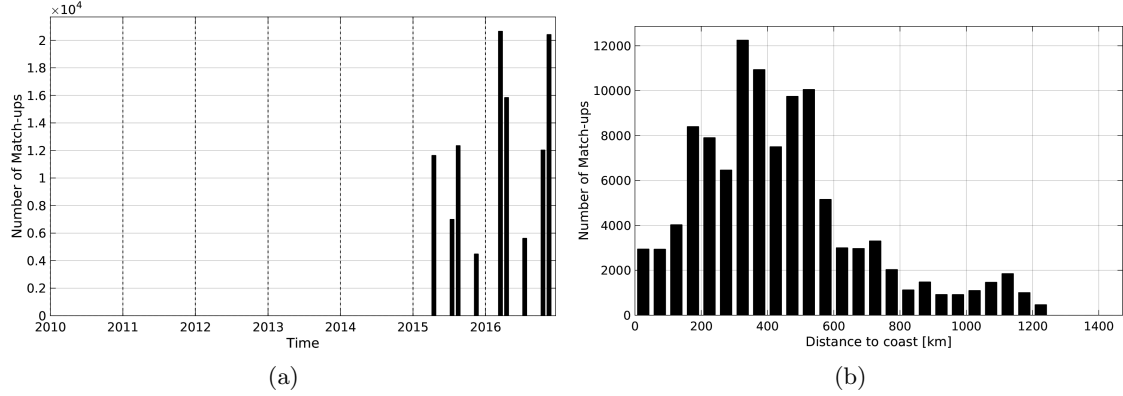
Figure 1: Number of match-ups between TSG-GOSUD-Research-vessel and SMAP-L3-RSS-V2-MONTHLY-0.25DEG-40KM SSS as a function of time (a) and as function of the distance to coast (b) over the Equatorial Ocean 10N-10S Pi-MEP region and for the full satellite product period.
