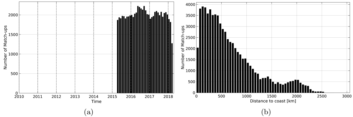
Figure 1: Number of match-ups between Argo and SMAP-L3-RSS-V2-MONTHLY-0.25DEG-40KM SSS as a function of time (a) and as function of the distance to coast (b) over the Equatorial Ocean 10N-10S Pi-MEP region and for the full satellite product period.
