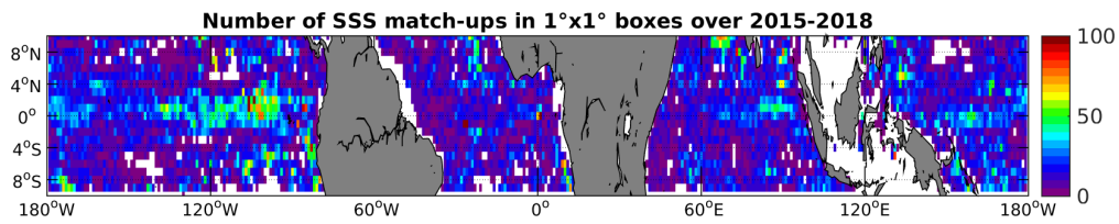
Figure 4: Number of SSS match-ups between Argo SSS and the SMAP-L3-RSS-V2-MONTHLY-0.25DEG-40KM SSS product for the Equatorial Ocean 10N-10S Pi-MEP region over 1^\circ \times 1^\circ boxes and for the full satellite product period.
