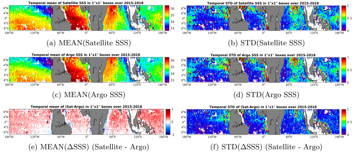
Figure 6: Temporal mean (left) and STD (right) of SSS from SMAP-L3-RSS-V2-MONTHLY-0.25DEG-40KM (top), Argo (middle), and of \Delta SSS (Satellite - Argo). Only match-up pairs are used to generate these maps.
