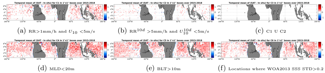
Figure 12: Temporal mean gridded over spatial boxes of size 1^\circ \times 1^\circ of \Delta SSS (SMAP-L3-RSS-V2-MONTHLY-0.25DEG-40KM - Argo) for 6 different subdatasets corresponding to: RR > 1\text{mm/h} and U_{10} < 5\text{m/s} (a), RR^{10d} > 5\text{mm/h} and U_{10}^{10d} < 5\text{m/s} (b), C1 U C2 (c), MLD < 20\text{m} (d), BLT > 10\text{m} (e), Locations where WOA2013 SSS STD > 0.2 (f).
