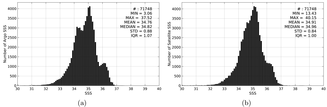
Figure 2: Histograms of SSS from Argo (a) and SMAP-L3-RSS-V2-MONTHLY-0.25DEG-40KM (b) considering all match-up pairs per bins of 0.1 over the Equatorial Ocean 10N-10S Pi-MEP region and for the full satellite product period.
