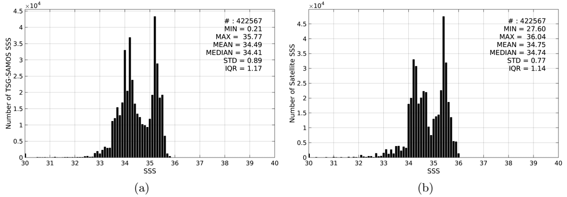
Figure 2: Histograms of SSS from TSG-SAMOS (a) and SMAP-L3-RSS-V2-MONTHLY-70KM (b) considering all match-up pairs per bins of 0.1 over the Equatorial Ocean 10N-10S Pi-MEP region and for the full satellite product period.
