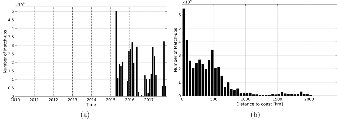
Figure 1: Number of match-ups between TSG-SAMOS and SMAP-L3-RSS-V2-MONTHLY-70KM SSS as a function of time (a) and as function of the distance to coast (b) over the Equatorial Ocean 10N-10S Pi-MEP region and for the full satellite product period.
