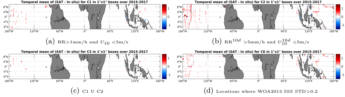
Figure 12: Temporal mean gridded over spatial boxes of size 1^\circ \times 1^\circ of \Delta SSS (SMAP-L3-RSS-V2-MONTHLY-70KM - TSG-SAMOS) for 4 different subdatasets corresponding to: RR > 1\text{mm/h} and U_{10} < 5\text{m/s} (a), RR^{10d} > 5\text{mm/h} and U_{10}^{10d} < 5\text{m/s} (b), C1 U C2 (c), Locations where WOA2013 SSS STD > 0.2 (d).
