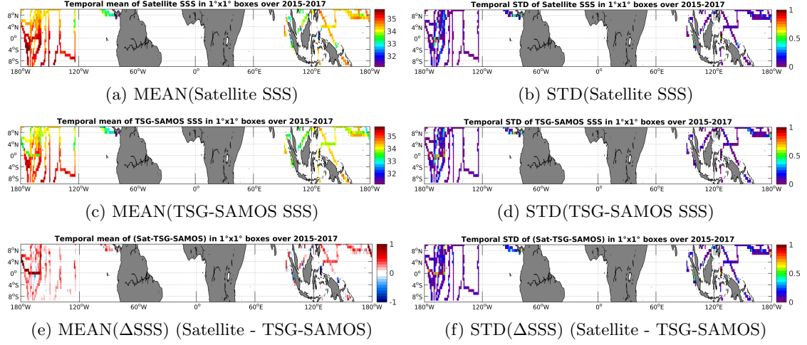
Figure 6: Temporal mean (left) and STD (right) of SSS from SMAP-L3-RSS-V2-MONTHLY-70KM (top), TSG-SAMOS (middle), and of \Delta SSS (Satellite - TSG-SAMOS). Only match-up pairs are used to generate these maps.
