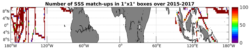
Figure 4: Number of SSS match-ups between TSG-SAMOS SSS and the SMAP-L3-RSS-V2-MONTHLY-70KM SSS product for the Equatorial Ocean 10N-10S Pi-MEP region over 1^\circ \times 1^\circ boxes and for the full satellite product period.
