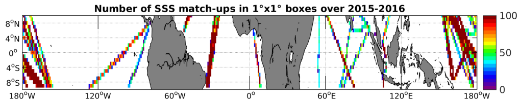
Figure 4: Number of SSS match-ups between TSG-LEGOS-DM SSS and the SMAP-L3-RSS-V2-MONTHLY-70KM SSS product for the Equatorial Ocean 10N-10S Pi-MEP region over 1^\circ \times 1^\circ boxes and for the full satellite product period.
