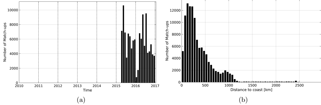
Figure 1: Number of match-ups between TSG-LEGOS-DM and SMAP-L3-RSS-V2-MONTHLY-70KM SSS as a function of time (a) and as function of the distance to coast (b) over the Equatorial Ocean 10N-10S Pi-MEP region and for the full satellite product period.
