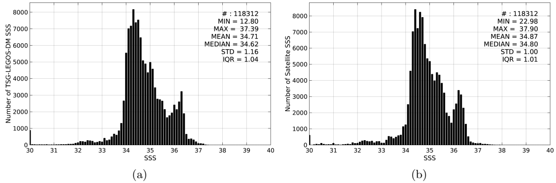
Figure 2: Histograms of SSS from TSG-LEGOS-DM (a) and SMAP-L3-RSS-V2-MONTHLY-70KM (b) considering all match-up pairs per bins of 0.1 over the Equatorial Ocean 10N-10S Pi-MEP region and for the full satellite product period.
