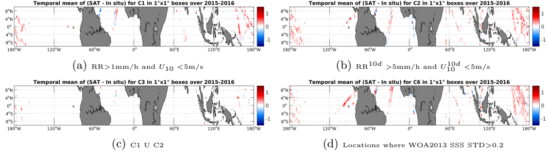
Figure 12: Temporal mean gridded over spatial boxes of size 1^\circ \times 1^\circ of \Delta SSS (SMAP-L3-RSS-V2-MONTHLY-70KM - TSG-LEGOS-DM) for 4 different subdatasets corresponding to: RR > 1 mm/h and U_{10} < 5 m/s (a), RR^{10d} > 5 mm/h and U_{10}^{10d} < 5 m/s (b), C1 U C2 (c), Locations where WOA2013 SSS STD > 0.2 (d).
