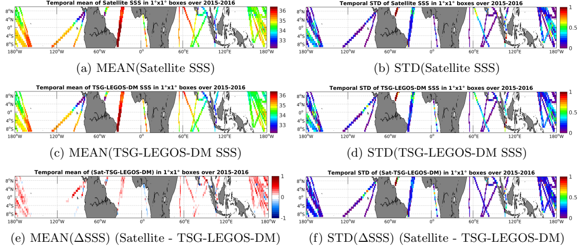
Figure 6: Temporal mean (left) and STD (right) of SSS from SMAP-L3-RSS-V2-MONTHLY-70KM (top), TSG-LEGOS-DM (middle), and of \Delta SSS (Satellite - TSG-LEGOS-DM). Only match-up pairs are used to generate these maps.
