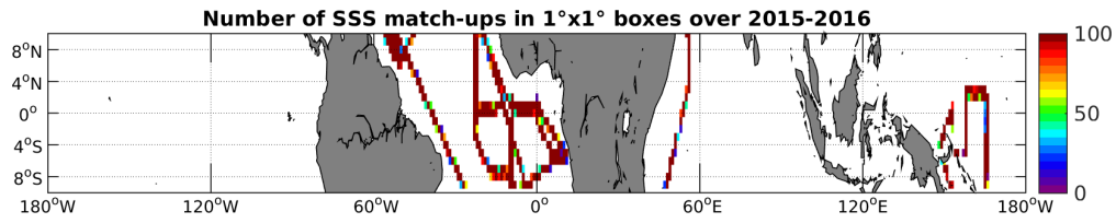
Figure 4: Number of SSS match-ups between TSG-GOSUD-Research-vessel SSS and the SMAP-L3-RSS-V2-MONTHLY-70KM SSS product for the Equatorial Ocean 10N-10S Pi-MEP region over 1°x1° boxes and for the full satellite product period.
