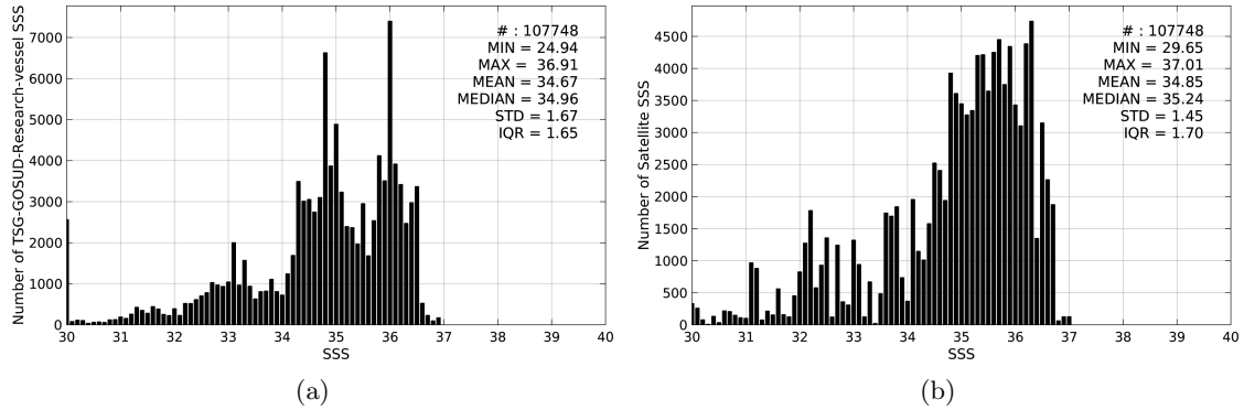
Figure 2: Histograms of SSS from TSG-GOSUD-Research-vessel (a) and SMAP-L3-RSS-V2-MONTHLY-70KM (b) considering all match-up pairs per bins of 0.1 over the Equatorial Ocean 10N-10S Pi-MEP region and for the full satellite product period.
