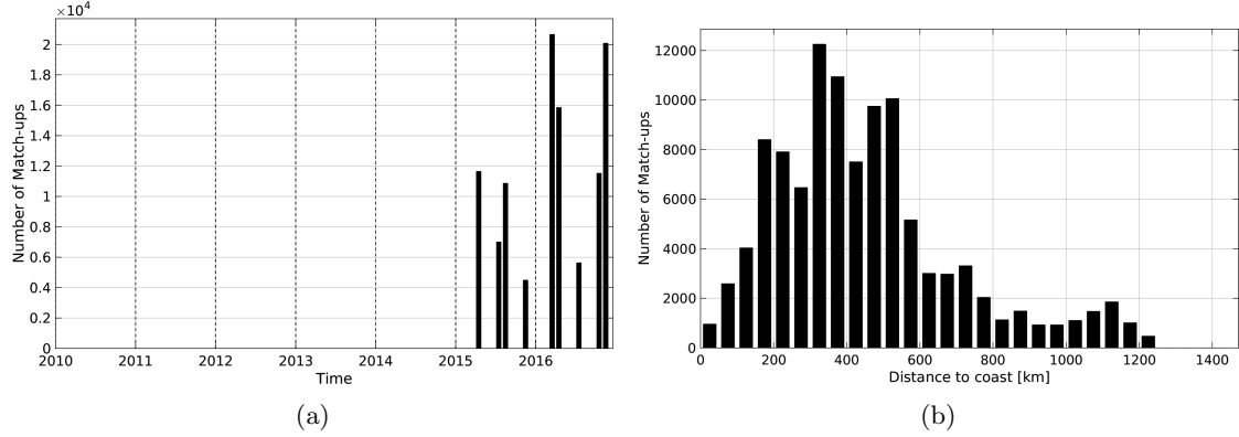
Figure 1: Number of match-ups between TSG-GOSUD-Research-vessel and SMAP-L3-RSS-V2-MONTHLY-70KM SSS as a function of time (a) and as function of the distance to coast (b) over the Equatorial Ocean 10N-10S Pi-MEP region and for the full satellite product period.
