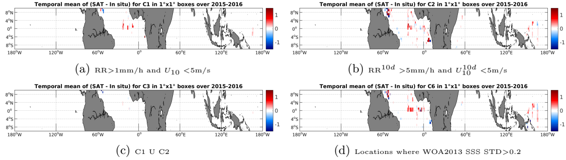
Figure 12: Temporal mean gridded over spatial boxes of size 1^\circ \times 1^\circ of \Delta SSS (SMAP-L3-RSS-V2-MONTHLY-70KM - TSG-GOSUD-Research-vessel) for 4 different subdatasets corresponding to: RR > 1 mm/h and U_{10} < 5 m/s (a), RR^{10d} > 5 mm/h and U_{10}^{10d} < 5 m/s (b), C1 U C2 (c), Locations where WOA2013 SSS STD > 0.2 (d).
