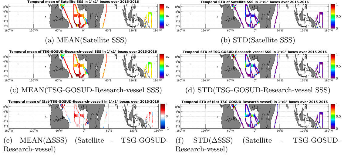
Figure 6: Temporal mean (left) and STD (right) of SSS from SMAP-L3-RSS-V2-MONTHLY-70KM (top), TSG-GOSUD-Research-vessel (middle), and of \Delta SSS (Satellite - TSG-GOSUD-Research-vessel). Only match-up pairs are used to generate these maps.
