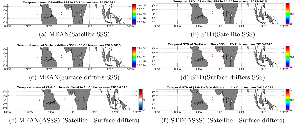
Figure 5: Temporal mean (left) and STD (right) of SSS from SMAP-L3-RSS-V2-MONTHLY-70KM (top), Surface drifters (middle), and of \Delta SSS (Satellite - Surface drifters). Only match-up pairs are used to generate these maps.
