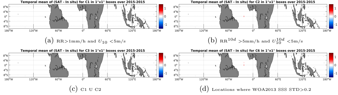
Figure 11: Temporal mean gridded over spatial boxes of size 1^\circ \times 1^\circ of \Delta SSS (SMAP-L3-RSS-V2-MONTHLY-70KM - Surface drifters) for 4 different subdatasets corresponding to: RR > 1\text{mm/h} and U_{10} < 5\text{m/s} (a), RR^{10d} > 5\text{mm/h} and U_{10}^{10d} < 5\text{m/s} (b), C1 U C2 (c), Locations where WOA2013 SSS STD > 0.2 (d).
