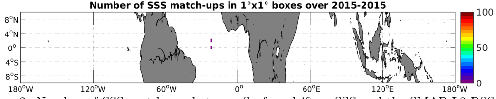
Figure 3: Number of SSS match-ups between Surface drifters SSS and the SMAP-L3-RSS-V2-MONTHLY-70KM SSS product for the Equatorial Ocean 10N-10S Pi-MEP region over 1^\circ \times 1^\circ boxes and for the full satellite product period.
