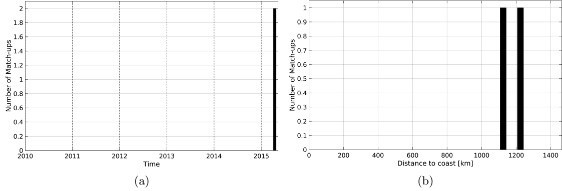
Figure 1: Number of match-ups between Surface drifters and SMAP-L3-RSS-V2-MONTHLY-70KM SSS as a function of time (a) and as function of the distance to coast (b) over the Equatorial Ocean 10N-10S Pi-MEP region and for the full satellite product period.
